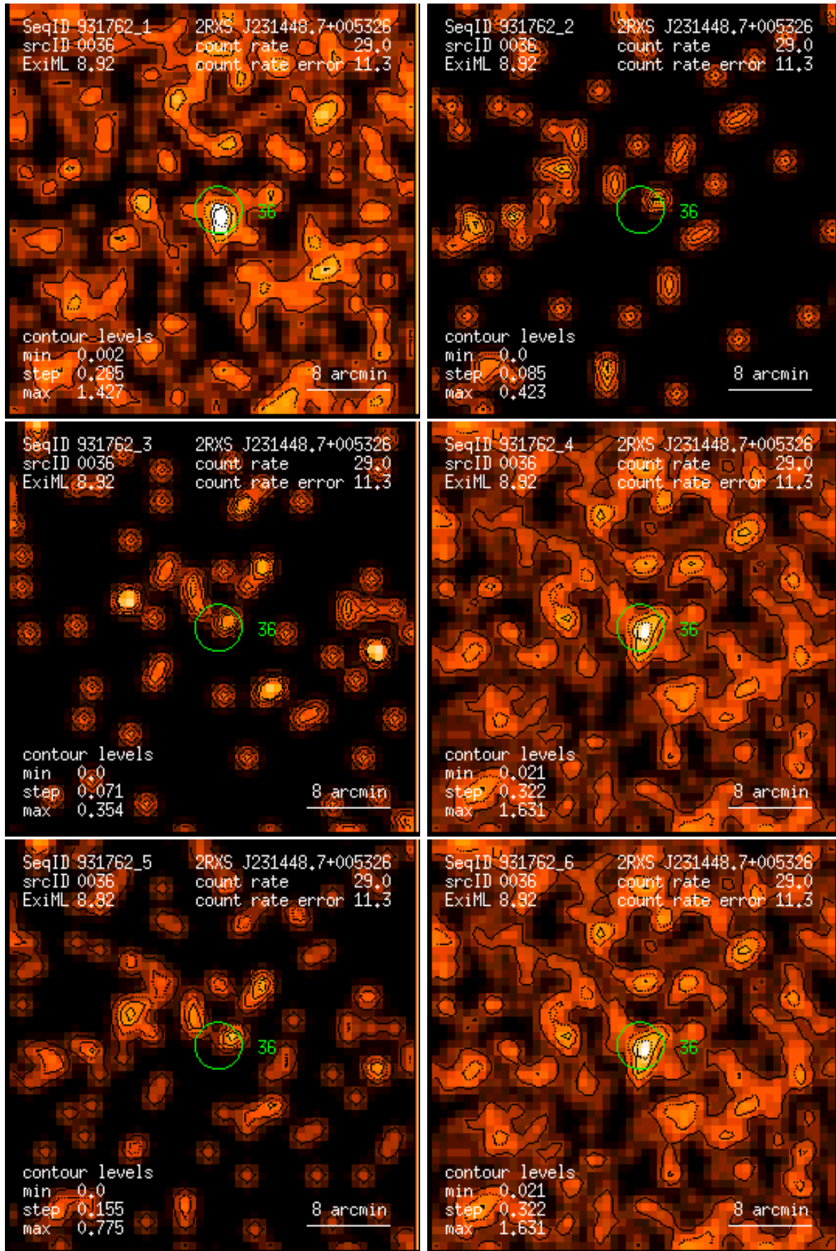
Figure 36: RASS 931762: detection 0036: band rate images, Gaussian filter: (1) PSPC channels 11 – 41, (2) 52 – 90, (3) 91 – 201, (4) 11 – 235, (5) 52 – 201, (6) 11 – 201. Broad band rates in counts/ks. Band rate contour levels in counts/ks/arcmin 2 .
