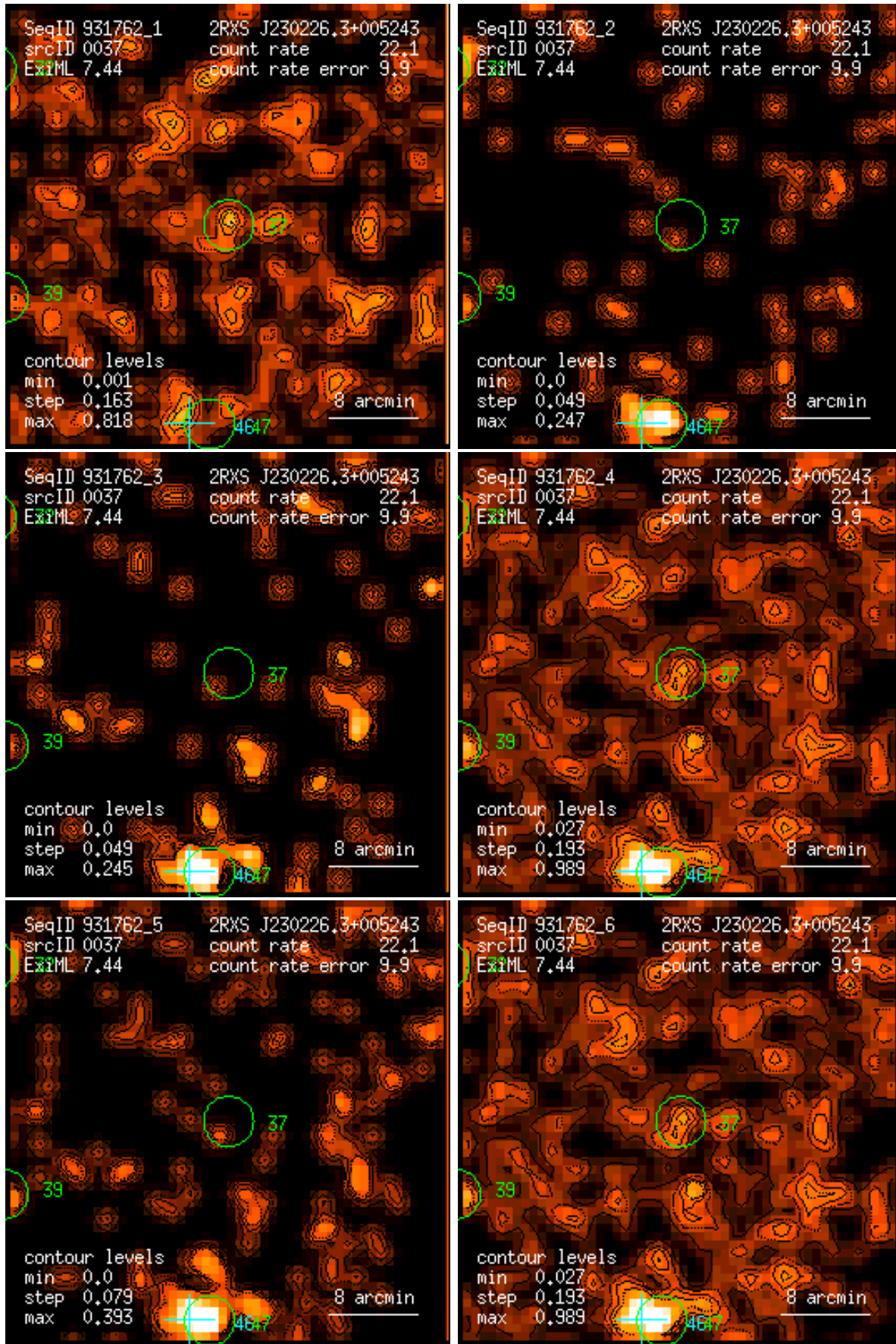
Figure 37: RASS 931762: detection 0037: band rate images, Gaussian filter: (1) PSPC channels 11 – 41, (2) 52 – 90, (3) 91 – 201, (4) 11 – 235, (5) 52 – 201, (6) 11 – 201. Broad band rates in counts/ks. Band rate contour levels in counts/ks/arcmin 2 .
