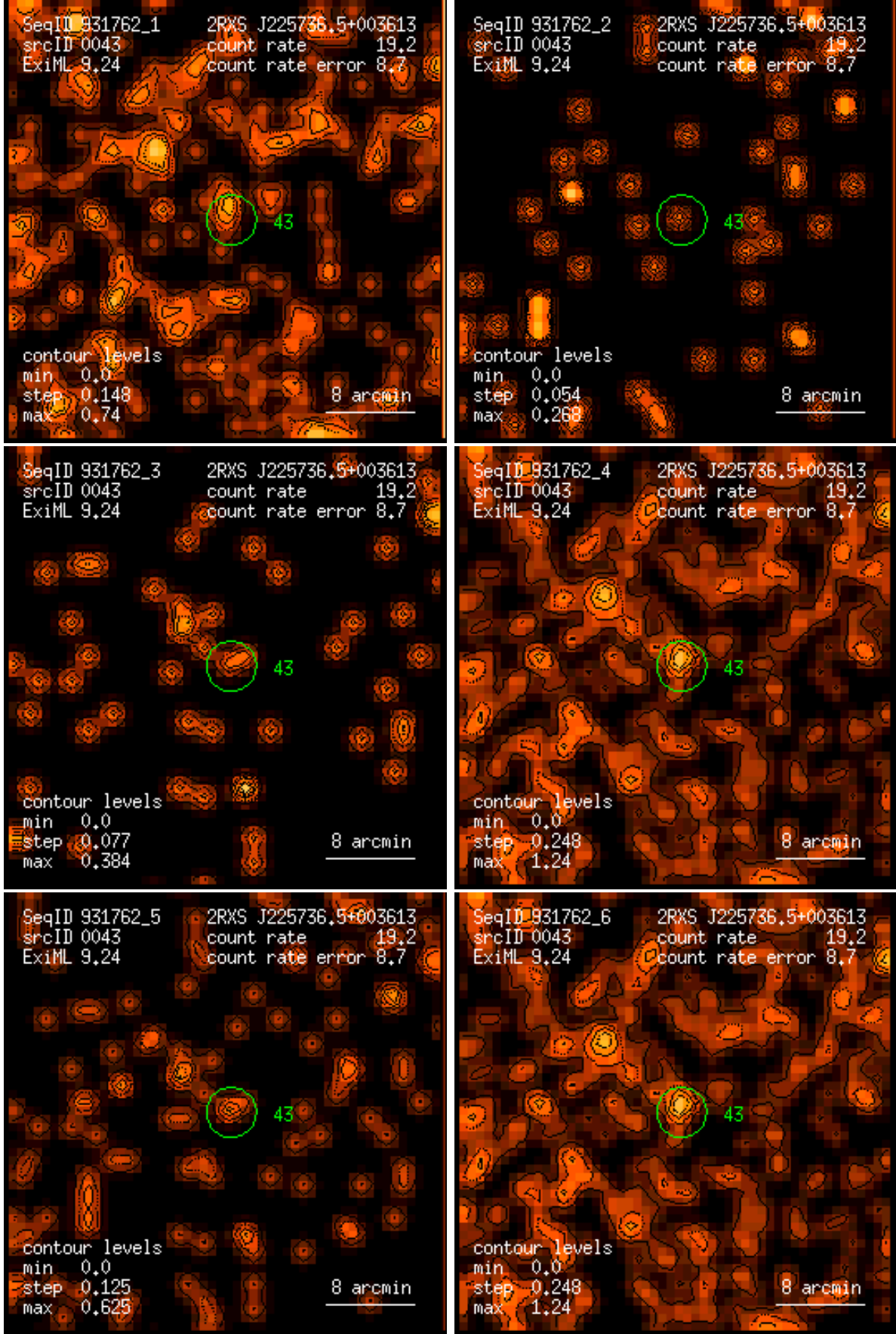
Figure 43: RASS 931762: detection 0043: band rate images, Gaussian filter: (1) PSPC channels 11 – 41, (2) 52 – 90, (3) 91 – 201, (4) 11 – 235, (5) 52 – 201, (6) 11 – 201. Broad band rates in counts/ks. Band rate contour levels in counts/ks/arcmin 2 .
