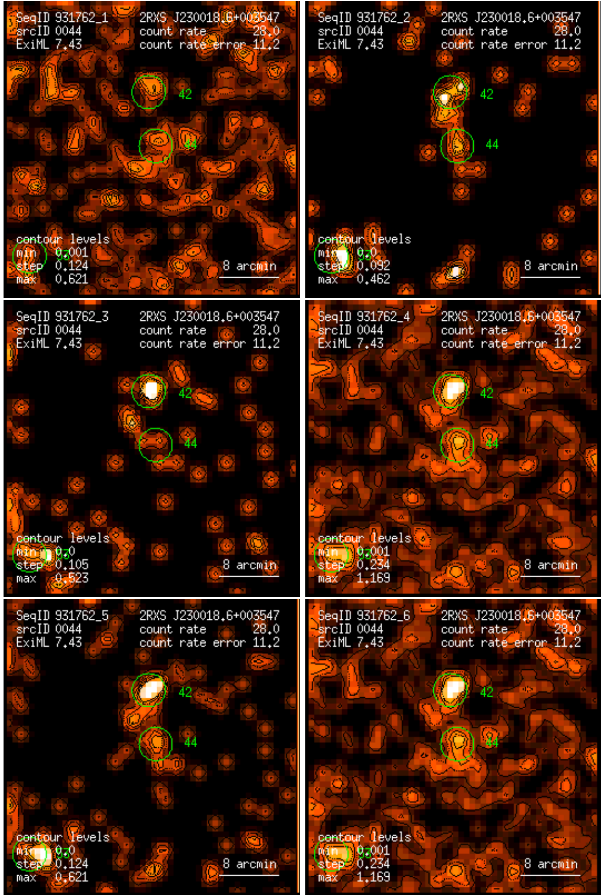
Figure 44: RASS 931762: detection 0044: band rate images, Gaussian filter: (1) PSPC channels 11 – 41, (2) 52 – 90, (3) 91 – 201, (4) 11 – 235, (5) 52 – 201, (6) 11 – 201. Broad band rates in counts/ks. Band rate contour levels in counts/ks/arcmin 2 .
