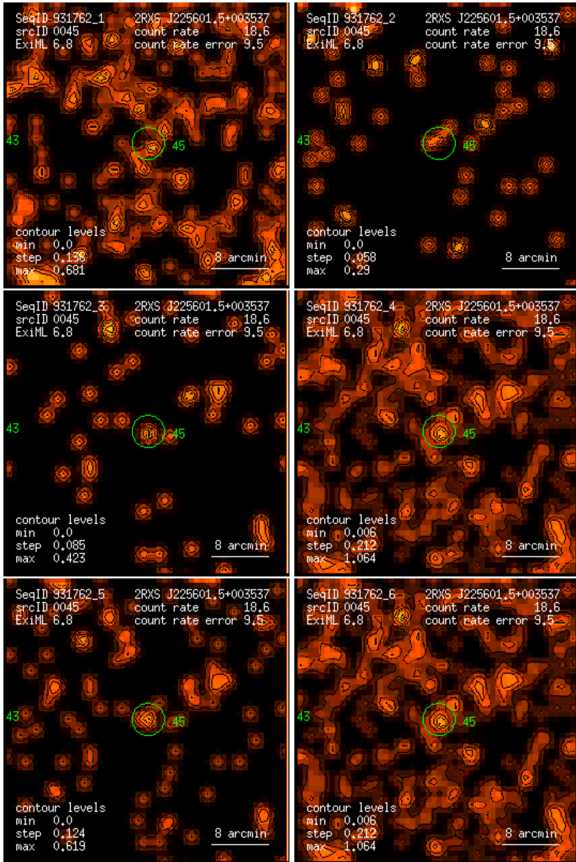
Figure 45: RASS 931762: detection 0045: band rate images, Gaussian filter: (1) PSPC channels 11 – 41, (2) 52 – 90, (3) 91 – 201, (4) 11 – 235, (5) 52 – 201, (6) 11 – 201. Broad band rates in counts/ks. Band rate contour levels in counts/ks/arcmin 2 .
