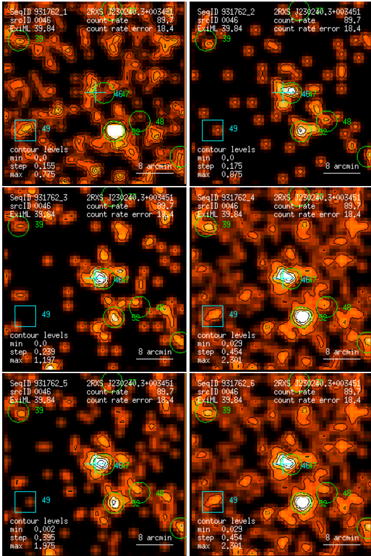
Figure 46: RASS 931762: detection 0046: band rate images, Gaussian filter: (1) PSPC channels 11 – 41, (2) 52 – 90, (3) 91 – 201, (4) 11 – 235, (5) 52 – 201, (6) 11 – 201. Broad band rates in counts/ks. Band rate contour levels in counts/ks/arcmin 2 .
