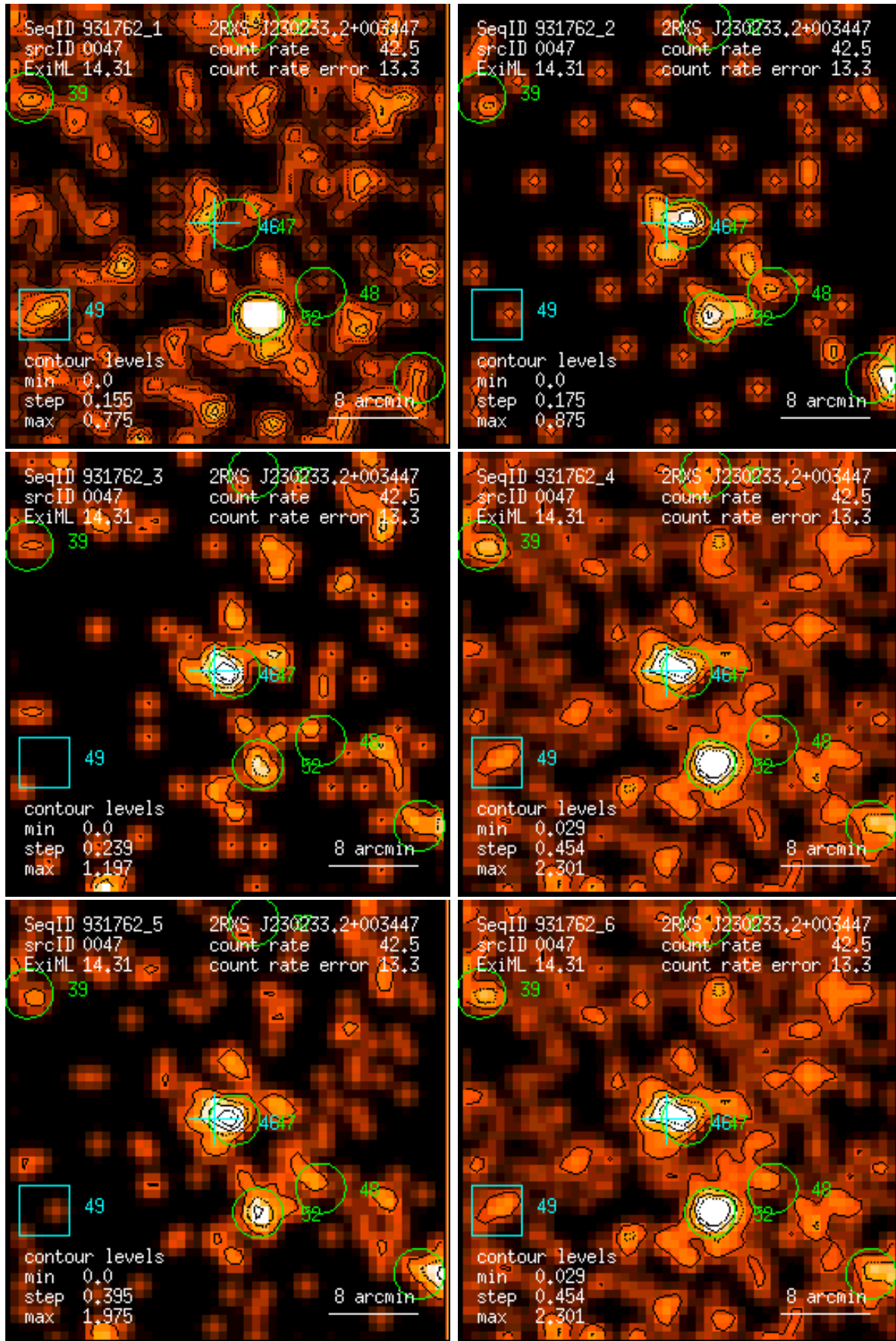
Figure 47: RASS 931762: detection 0047: band rate images, Gaussian filter: (1) PSPC channels 11 – 41, (2) 52 – 90, (3) 91 – 201, (4) 11 – 235, (5) 52 – 201, (6) 11 – 201. Broad band rates in counts/ks. Band rate contour levels in counts/ks/arcmin 2 .
