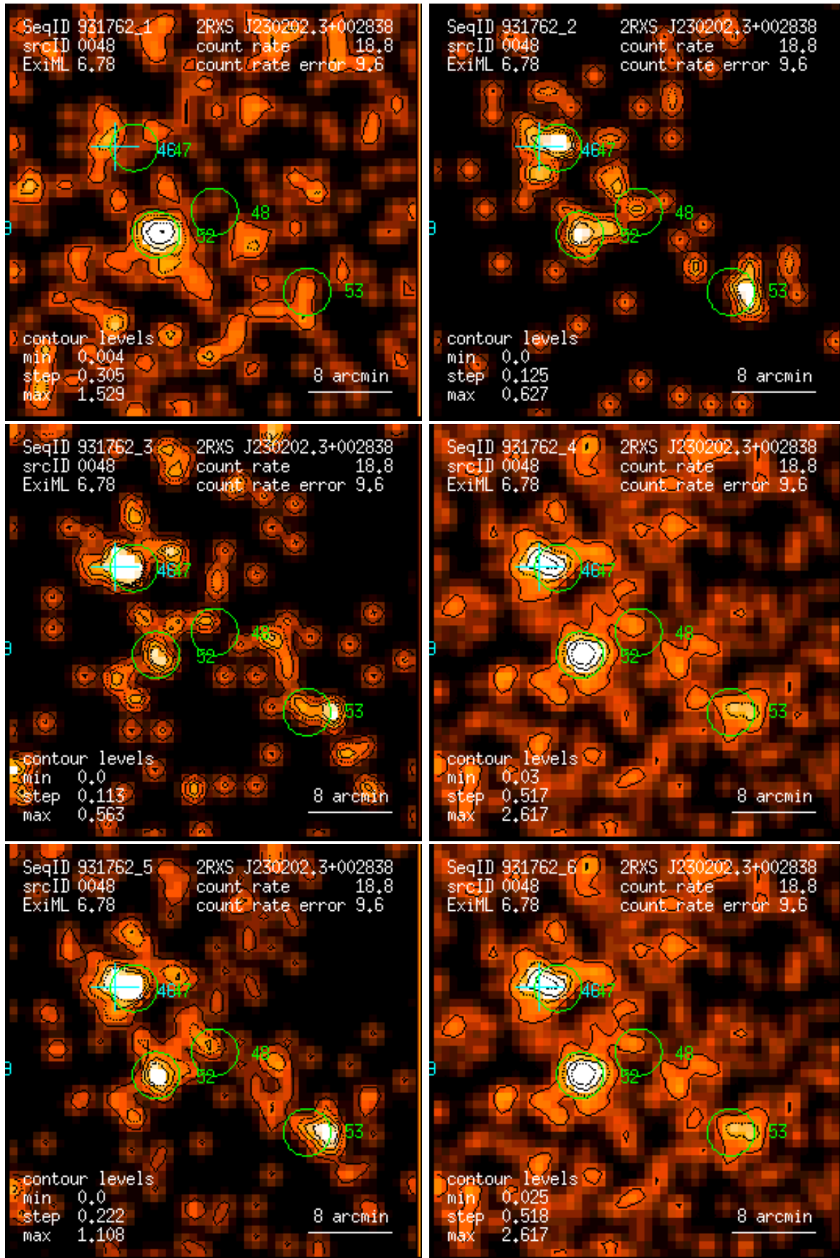
Figure 48: RASS 931762: detection 0048: band rate images, Gaussian filter: (1) PSPC channels 11 – 41, (2) 52 – 90, (3) 91 – 201, (4) 11 – 235, (5) 52 – 201, (6) 11 – 201. Broad band rates in counts/ks. Band rate contour levels in counts/ks/arcmin 2 .
