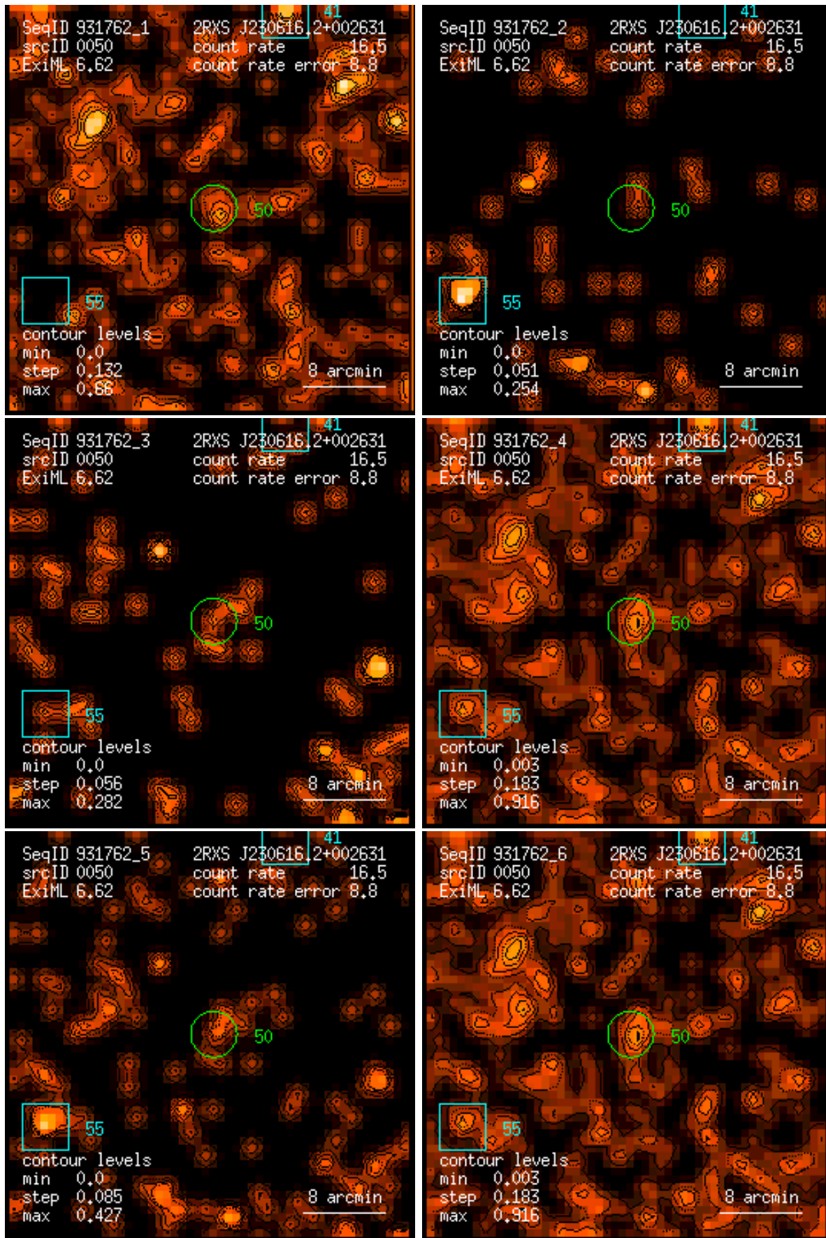
Figure 50: RASS 931762: detection 0050: band rate images, Gaussian filter: (1) PSPC channels 11 – 41, (2) 52 – 90, (3) 91 – 201, (4) 11 – 235, (5) 52 – 201, (6) 11 – 201. Broad band rates in counts/ks. Band rate contour levels in counts/ks/arcmin 2 .
