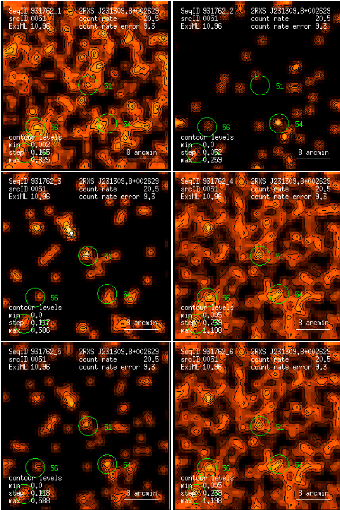
Figure 51: RASS 931762: detection 0051: band rate images, Gaussian filter: (1) PSPC channels 11 – 41, (2) 52 – 90, (3) 91 – 201, (4) 11 – 235, (5) 52 – 201, (6) 11 – 201. Broad band rates in counts/ks. Band rate contour levels in counts/ks/arcmin 2 .
