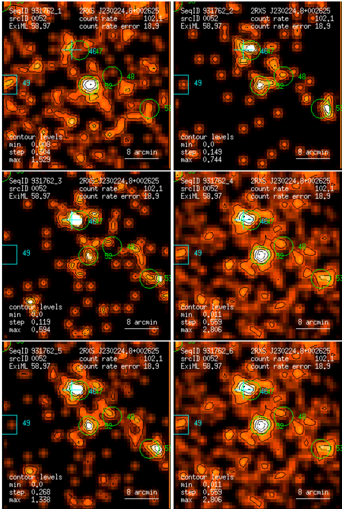
Figure 52: RASS 931762: detection 0052: band rate images, Gaussian filter: (1) PSPC channels 11 – 41, (2) 52 – 90, (3) 91 – 201, (4) 11 – 235, (5) 52 – 201, (6) 11 – 201. Broad band rates in counts/ks. Band rate contour levels in counts/ks/arcmin 2 .
