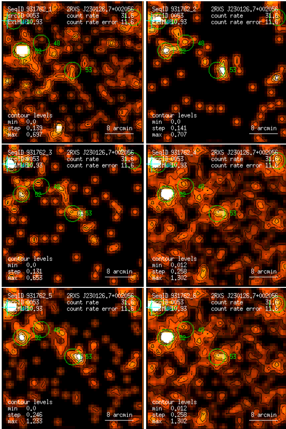
Figure 53: RASS 931762: detection 0053: band rate images, Gaussian filter: (1) PSPC channels 11 – 41, (2) 52 – 90, (3) 91 – 201, (4) 11 – 235, (5) 52 – 201, (6) 11 – 201. Broad band rates in counts/ks. Band rate contour levels in counts/ks/arcmin 2 .
