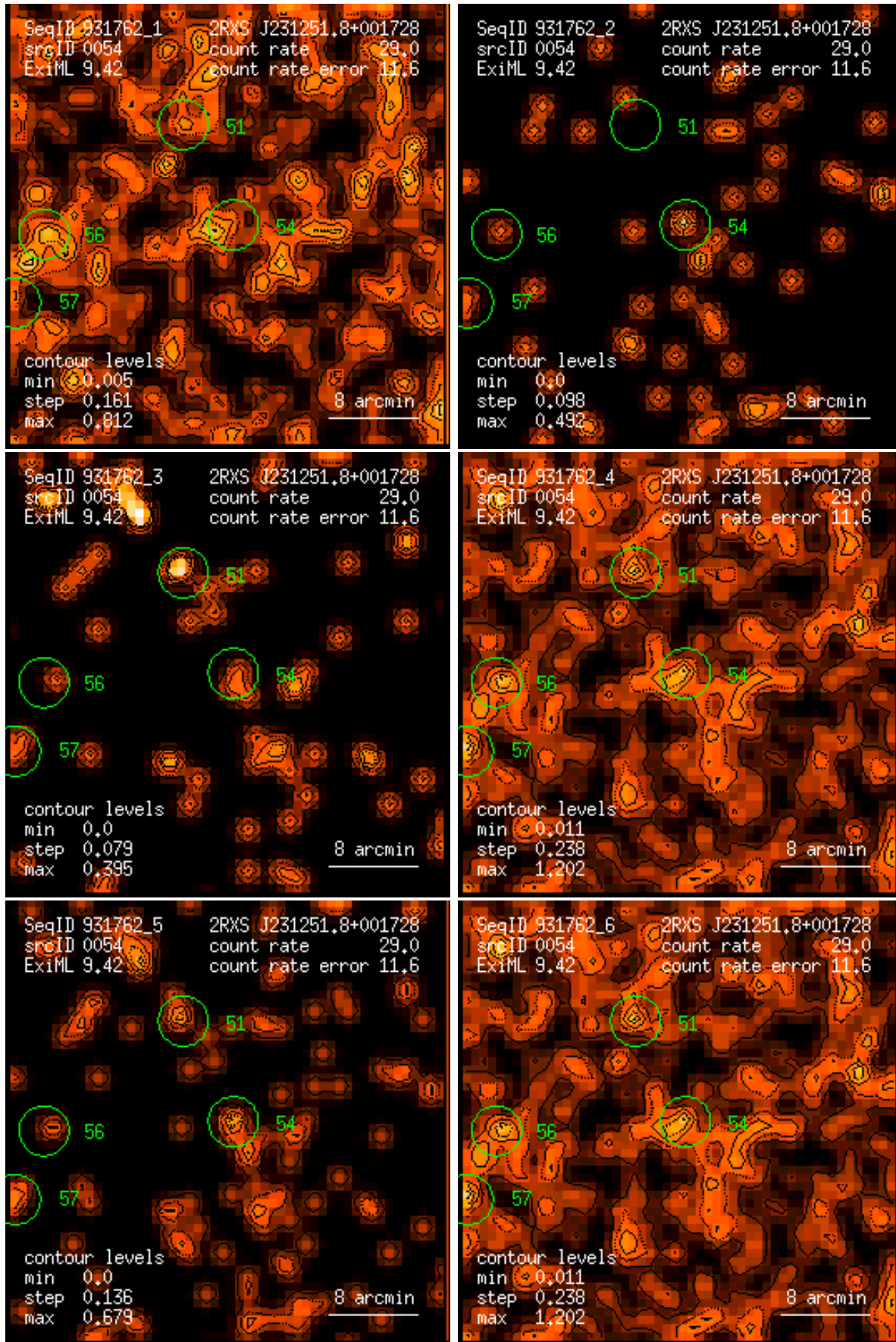
Figure 54: RASS 931762: detection 0054: band rate images, Gaussian filter: (1) PSPC channels 11 – 41, (2) 52 – 90, (3) 91 – 201, (4) 11 – 235, (5) 52 – 201, (6) 11 – 201. Broad band rates in counts/ks. Band rate contour levels in counts/ks/arcmin 2 .
