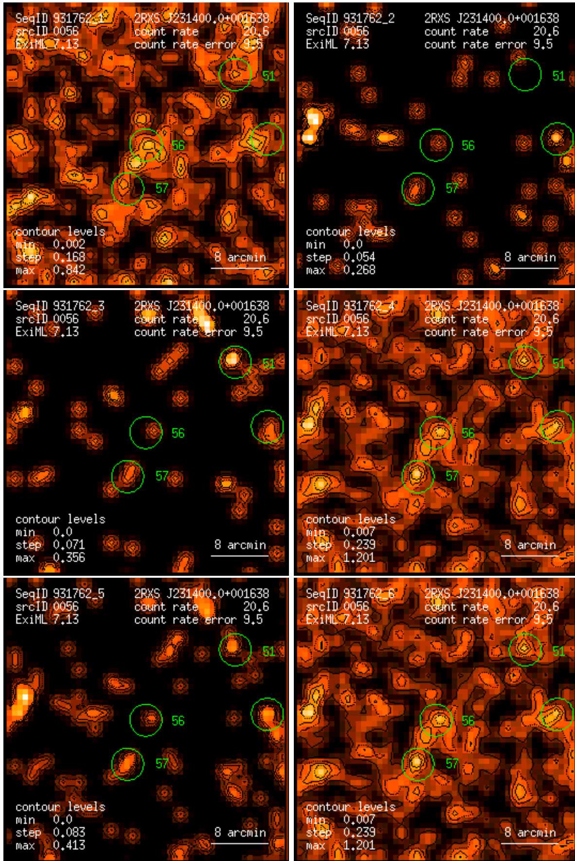
Figure 56: RASS 931762: detection 0056: band rate images, Gaussian filter: (1) PSPC channels 11 – 41, (2) 52 – 90, (3) 91 – 201, (4) 11 – 235, (5) 52 – 201, (6) 11 – 201. Broad band rates in counts/ks. Band rate contour levels in counts/ks/arcmin 2 .
