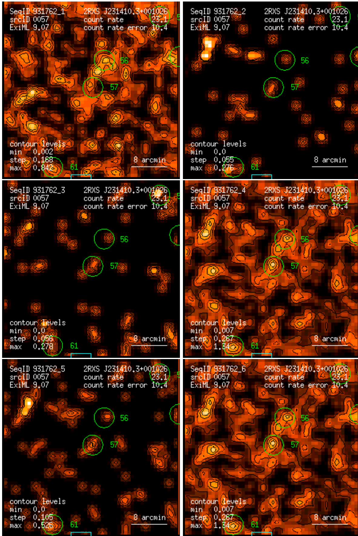
Figure 57: RASS 931762: detection 0057: band rate images, Gaussian filter: (1) PSPC channels 11 – 41, (2) 52 – 90, (3) 91 – 201, (4) 11 – 235, (5) 52 – 201, (6) 11 – 201. Broad band rates in counts/ks. Band rate contour levels in counts/ks/arcmin 2 .
