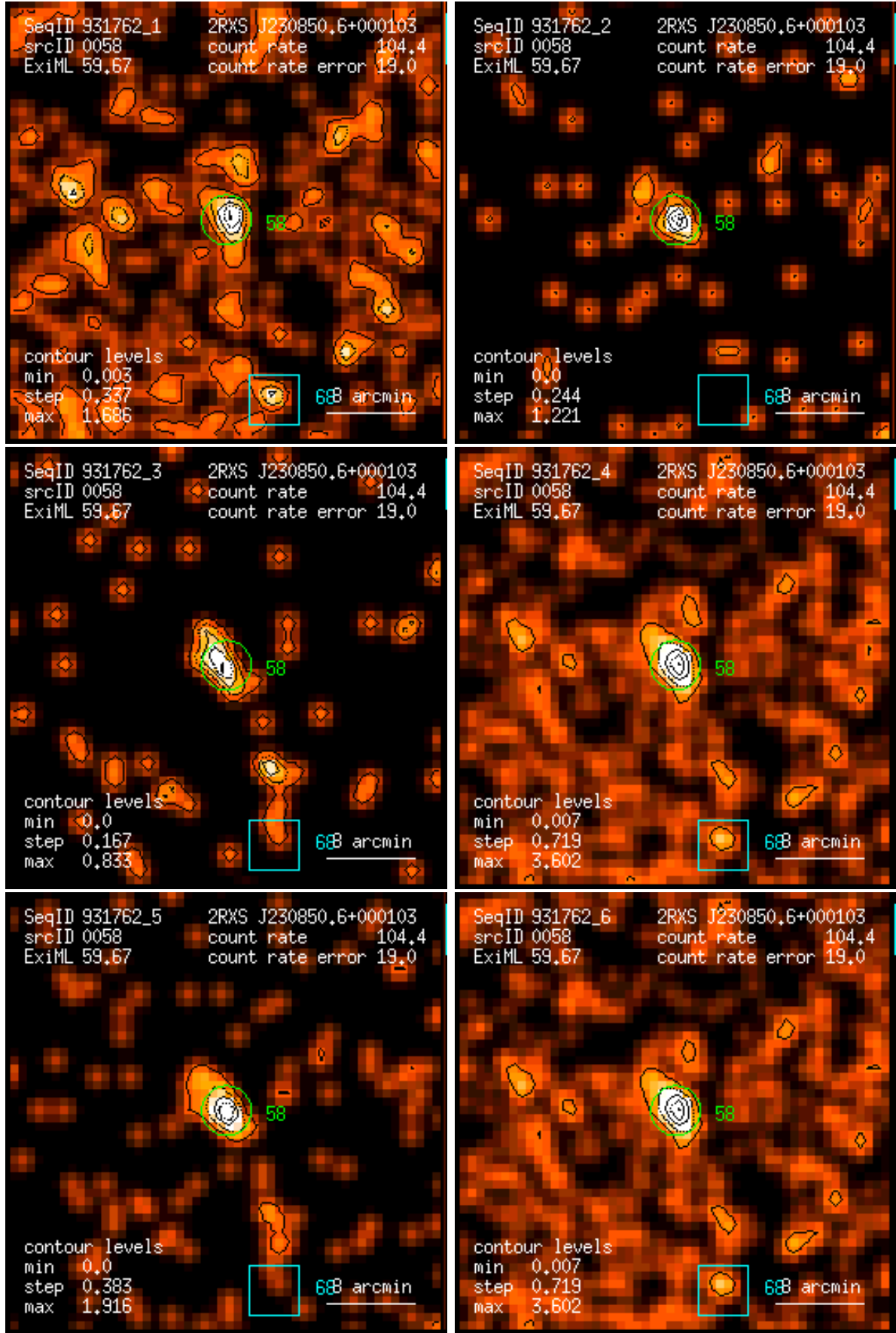
Figure 58: RASS 931762: detection 0058: band rate images, Gaussian filter: (1) PSPC channels 11 – 41, (2) 52 – 90, (3) 91 – 201, (4) 11 – 235, (5) 52 – 201, (6) 11 – 201. Broad band rates in counts/ks. Band rate contour levels in counts/ks/arcmin 2 .
