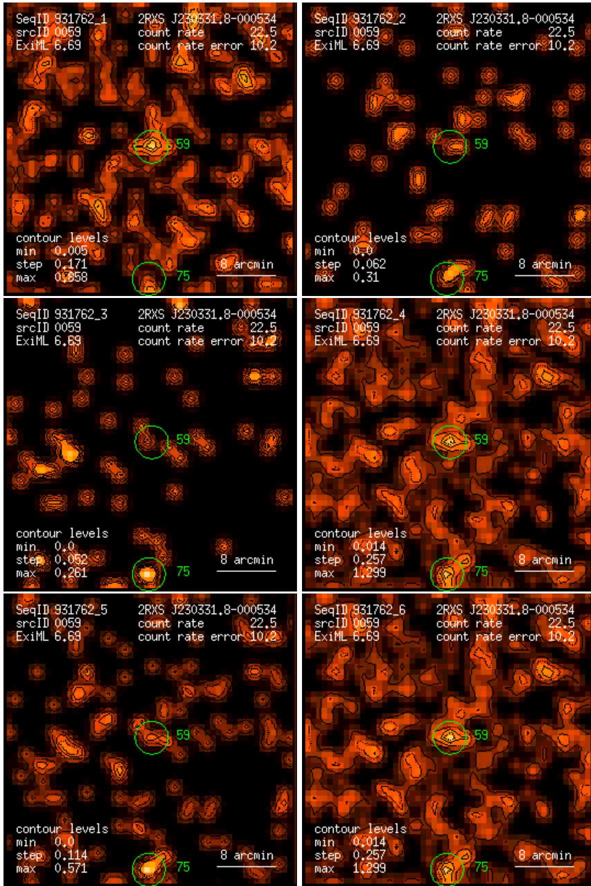
Figure 59: RASS 931762: detection 0059: band rate images, Gaussian filter: (1) PSPC channels 11 – 41, (2) 52 – 90, (3) 91 – 201, (4) 11 – 235, (5) 52 – 201, (6) 11 – 201. Broad band rates in counts/ks. Band rate contour levels in counts/ks/arcmin 2 .
