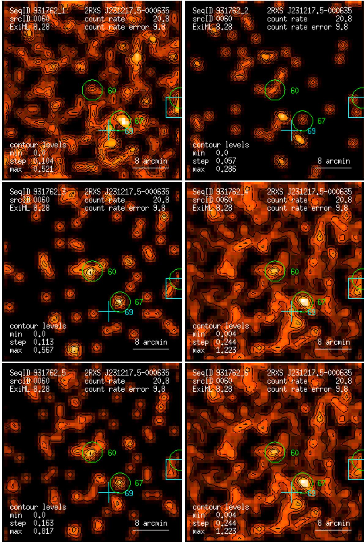
Figure 60: RASS 931762: detection 0060: band rate images, Gaussian filter: (1) PSPC channels 11 – 41, (2) 52 – 90, (3) 91 – 201, (4) 11 – 235, (5) 52 – 201, (6) 11 – 201. Broad band rates in counts/ks. Band rate contour levels in counts/ks/arcmin 2 .
