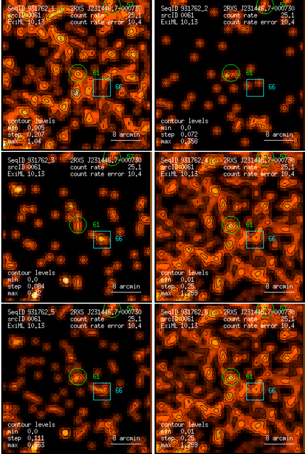
Figure 61: RASS 931762: detection 0061: band rate images, Gaussian filter: (1) PSPC channels 11 – 41, (2) 52 – 90, (3) 91 – 201, (4) 11 – 235, (5) 52 – 201, (6) 11 – 201. Broad band rates in counts/ks. Band rate contour levels in counts/ks/arcmin 2 .
