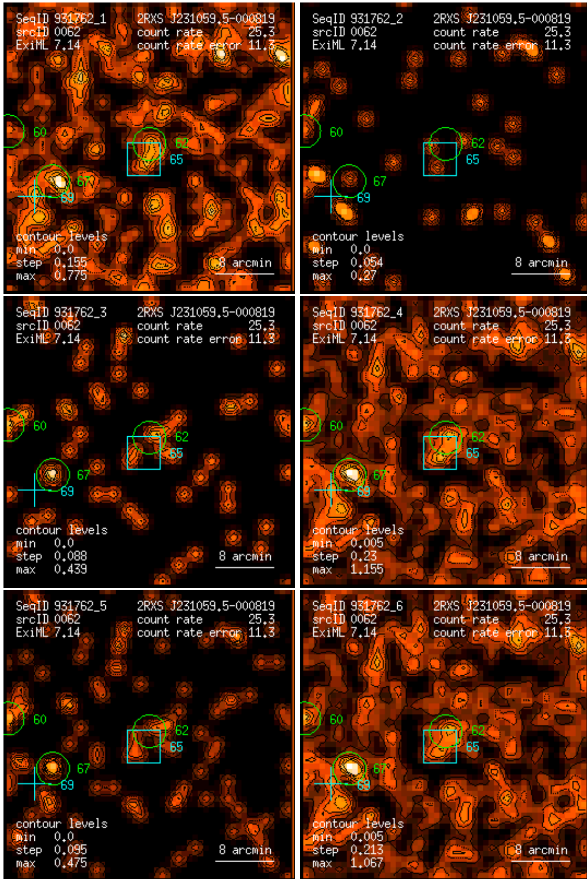
Figure 62: RASS 931762: detection 0062: band rate images, Gaussian filter: (1) PSPC channels 11 – 41, (2) 52 – 90, (3) 91 – 201, (4) 11 – 235, (5) 52 – 201, (6) 11 – 201. Broad band rates in counts/ks. Band rate contour levels in counts/ks/arcmin 2 .
