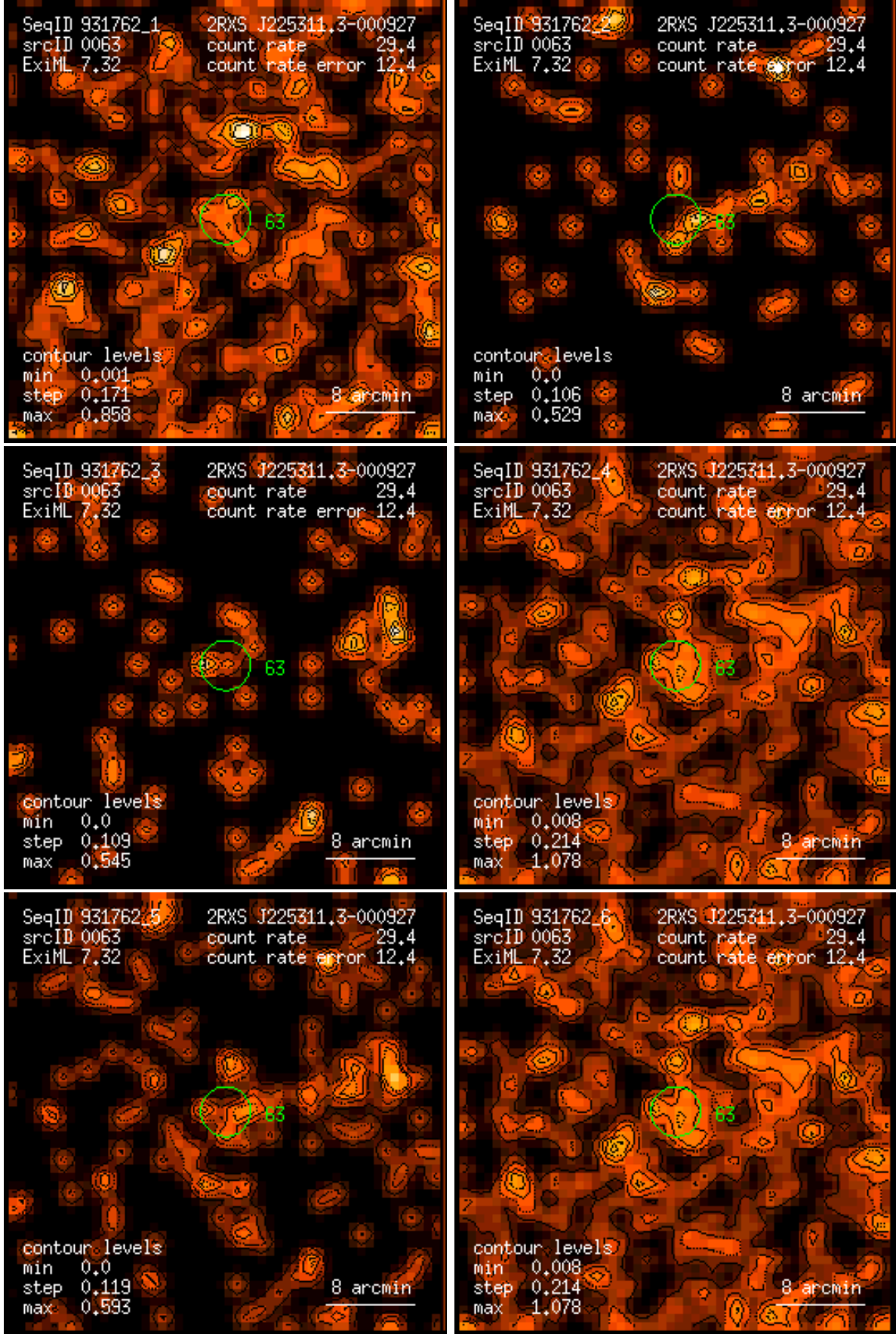
Figure 63: RASS 931762: detection 0063: band rate images, Gaussian filter: (1) PSPC channels 11 – 41, (2) 52 – 90, (3) 91 – 201, (4) 11 – 235, (5) 52 – 201, (6) 11 – 201. Broad band rates in counts/ks. Band rate contour levels in counts/ks/arcmin 2 .
