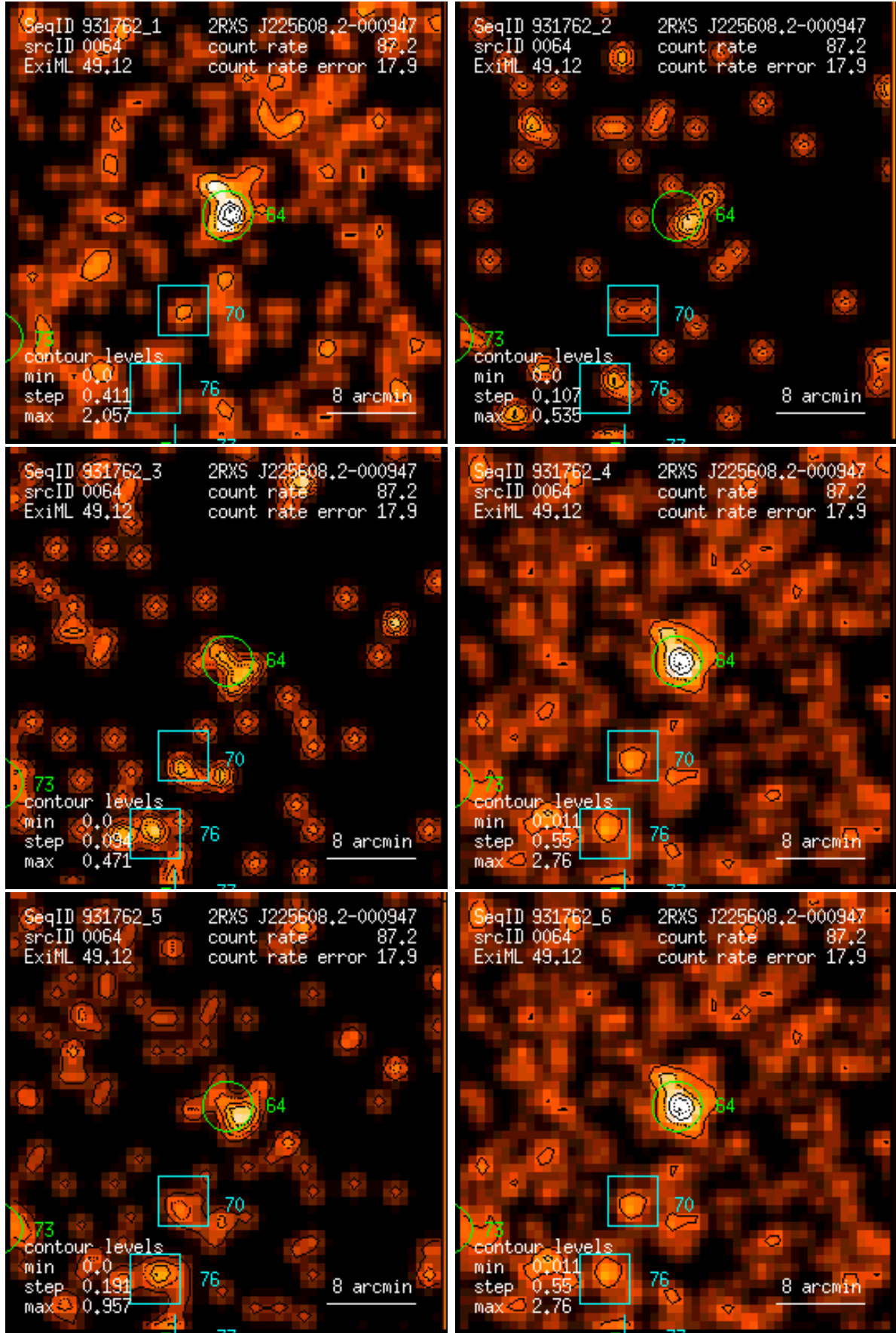
Figure 64: RASS 931762: detection 0064: band rate images, Gaussian filter: (1) PSPC channels 11 – 41, (2) 52 – 90, (3) 91 – 201, (4) 11 – 235, (5) 52 – 201, (6) 11 – 201. Broad band rates in counts/ks. Band rate contour levels in counts/ks/arcmin 2 .
