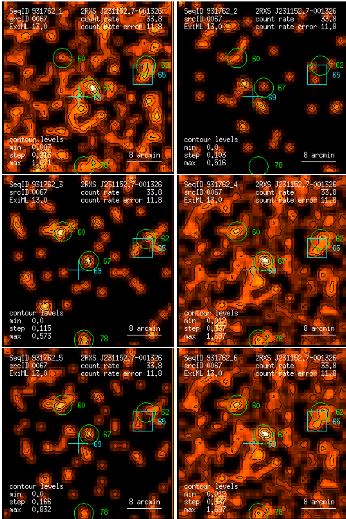
Figure 67: RASS 931762: detection 0067: band rate images, Gaussian filter: (1) PSPC channels 11 – 41, (2) 52 – 90, (3) 91 – 201, (4) 11 – 235, (5) 52 – 201, (6) 11 – 201. Broad band rates in counts/ks. Band rate contour levels in counts/ks/arcmin 2 .
