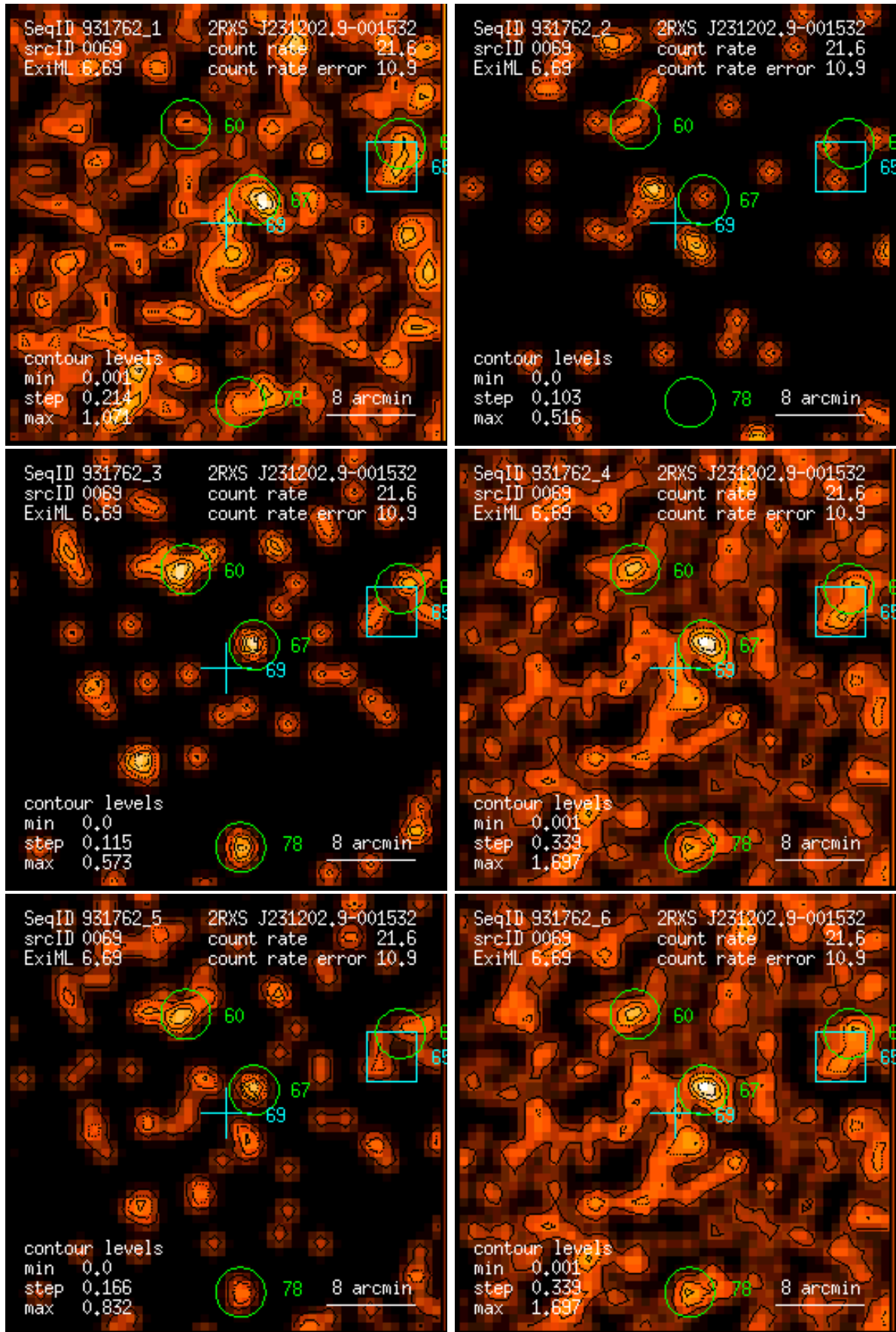
Figure 69: RASS 931762: detection 0069: band rate images, Gaussian filter: (1) PSPC channels 11 – 41, (2) 52 – 90, (3) 91 – 201, (4) 11 – 235, (5) 52 – 201, (6) 11 – 201. Broad band rates in counts/ks. Band rate contour levels in counts/ks/arcmin 2 .
