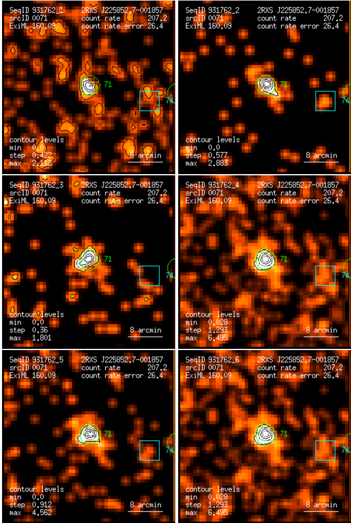
Figure 71: RASS 931762: detection 0071: band rate images, Gaussian filter: (1) PSPC channels 11 – 41, (2) 52 – 90, (3) 91 – 201, (4) 11 – 235, (5) 52 – 201, (6) 11 – 201. Broad band rates in counts/ks. Band rate contour levels in counts/ks/arcmin 2 .
