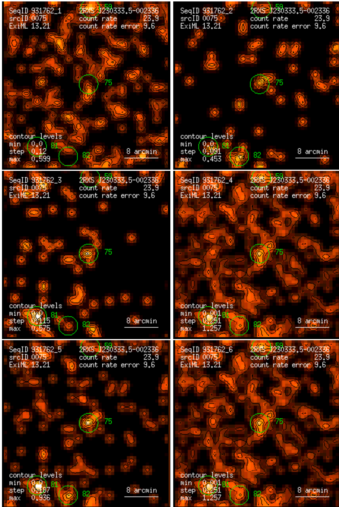
Figure 75: RASS 931762: detection 0075: band rate images, Gaussian filter: (1) PSPC channels 11 – 41, (2) 52 – 90, (3) 91 – 201, (4) 11 – 235, (5) 52 – 201, (6) 11 – 201. Broad band rates in counts/ks. Band rate contour levels in counts/ks/arcmin 2 .
