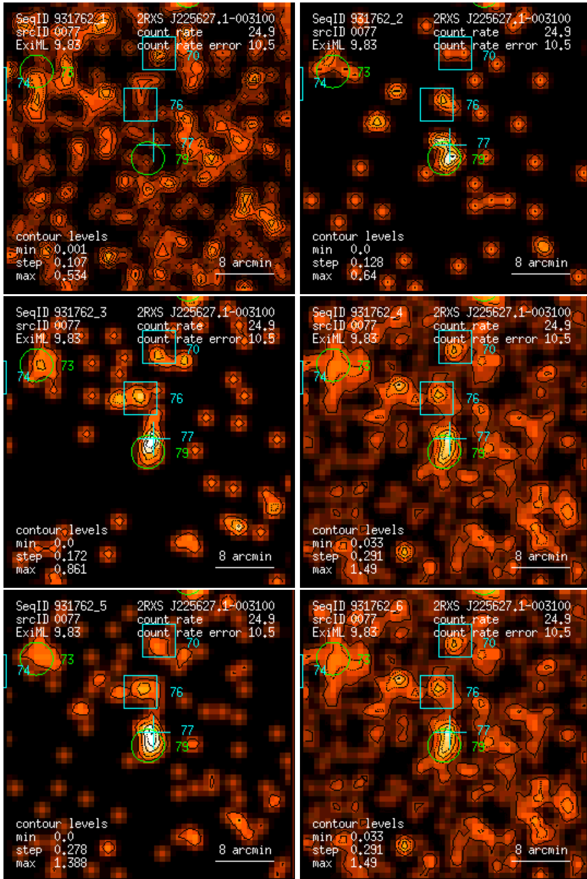
Figure 77: RASS 931762: detection 0077: band rate images, Gaussian filter: (1) PSPC channels 11 – 41, (2) 52 – 90, (3) 91 – 201, (4) 11 – 235, (5) 52 – 201, (6) 11 – 201. Broad band rates in counts/ks. Band rate contour levels in counts/ks/arcmin 2 .
