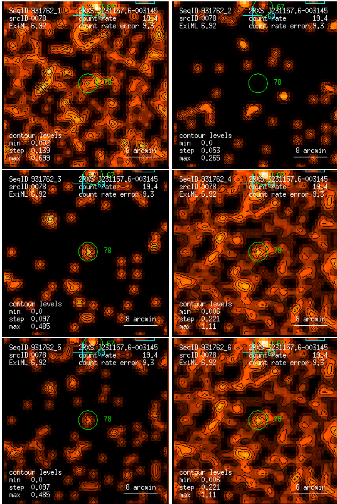
Figure 78: RASS 931762: detection 0078: band rate images, Gaussian filter: (1) PSPC channels 11 – 41, (2) 52 – 90, (3) 91 – 201, (4) 11 – 235, (5) 52 – 201, (6) 11 – 201. Broad band rates in counts/ks. Band rate contour levels in counts/ks/arcmin 2 .
