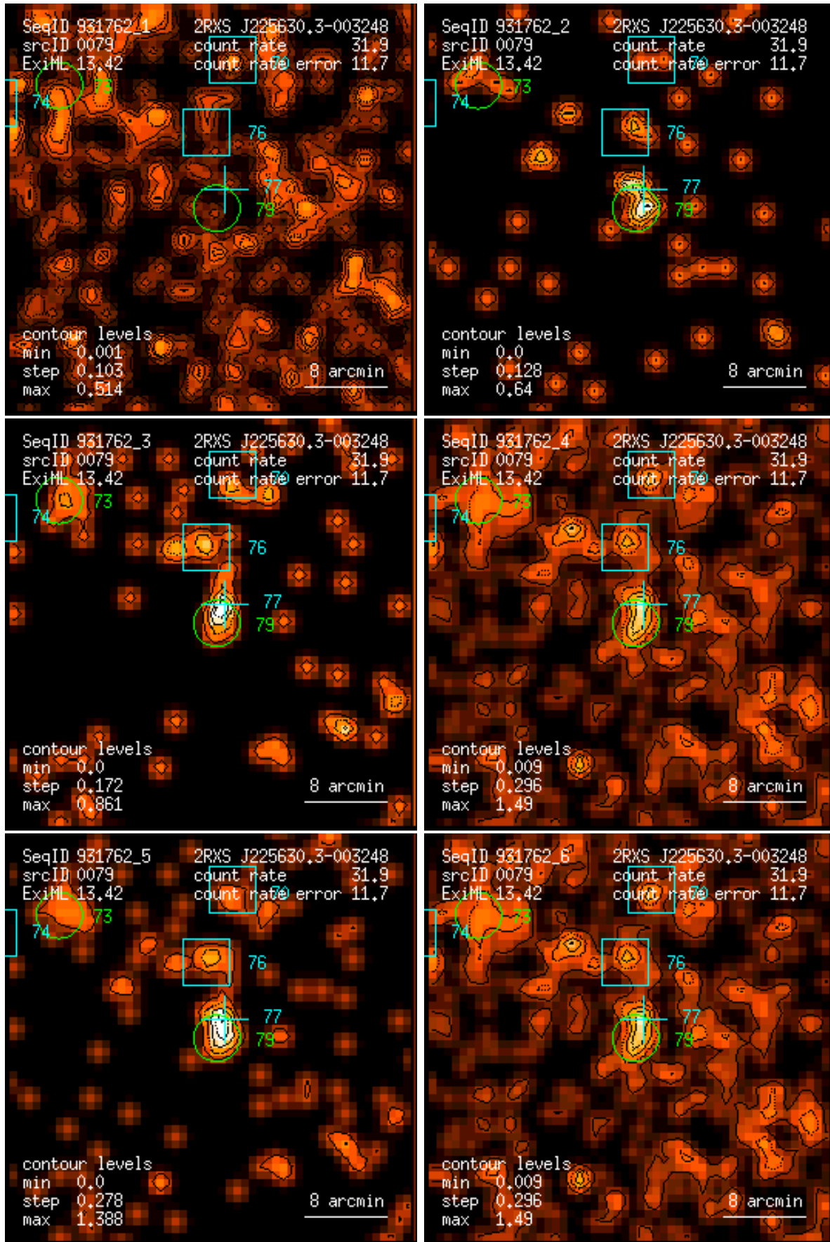
Figure 79: RASS 931762: detection 0079: band rate images, Gaussian filter: (1) PSPC channels 11 – 41, (2) 52 – 90, (3) 91 – 201, (4) 11 – 235, (5) 52 – 201, (6) 11 – 201. Broad band rates in counts/ks. Band rate contour levels in counts/ks/arcmin 2 .
