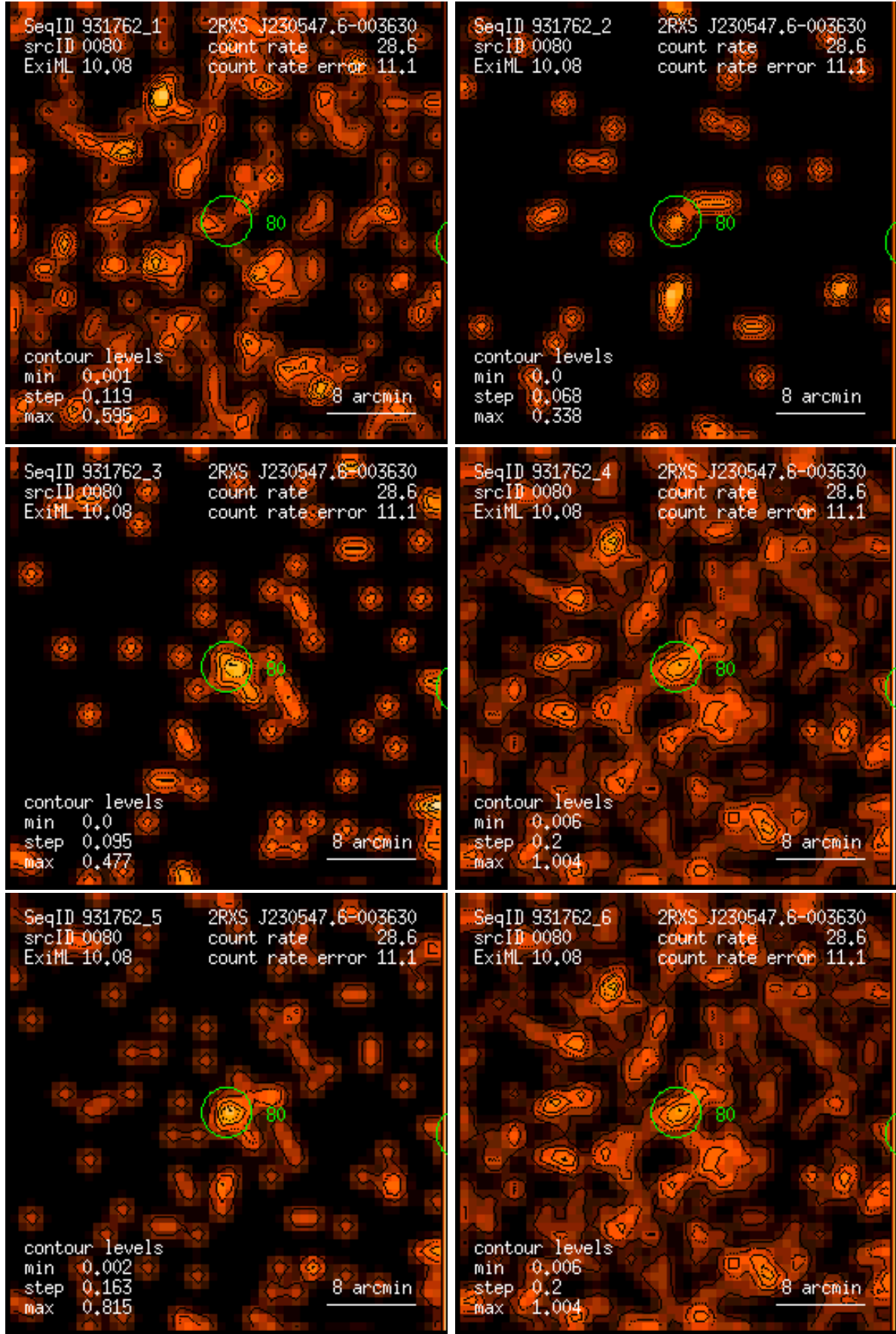
Figure 80: RASS 931762: detection 0080: band rate images, Gaussian filter: (1) PSPC channels 11 – 41, (2) 52 – 90, (3) 91 – 201, (4) 11 – 235, (5) 52 – 201, (6) 11 – 201. Broad band rates in counts/ks. Band rate contour levels in counts/ks/arcmin 2 .
