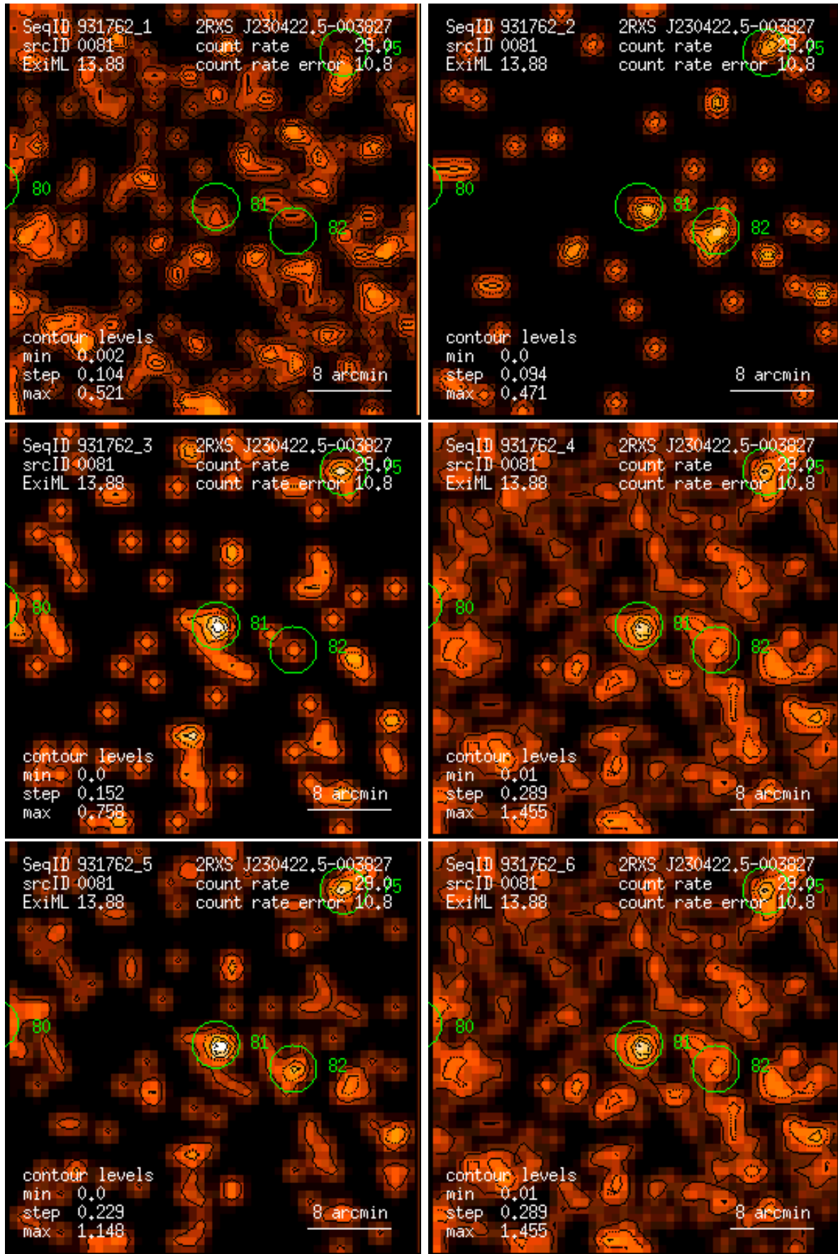
Figure 81: RASS 931762: detection 0081: band rate images, Gaussian filter: (1) PSPC channels 11 – 41, (2) 52 – 90, (3) 91 – 201, (4) 11 – 235, (5) 52 – 201, (6) 11 – 201. Broad band rates in counts/ks. Band rate contour levels in counts/ks/arcmin 2 .
