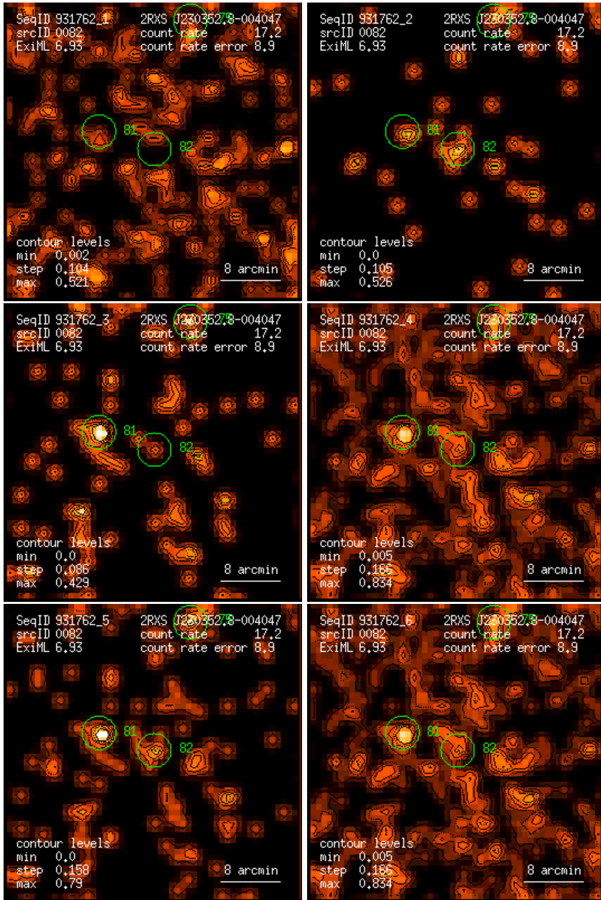
Figure 82: RASS 931762: detection 0082: band rate images, Gaussian filter: (1) PSPC channels 11 – 41, (2) 52 – 90, (3) 91 – 201, (4) 11 – 235, (5) 52 – 201, (6) 11 – 201. Broad band rates in counts/ks. Band rate contour levels in counts/ks/arcmin 2 .
