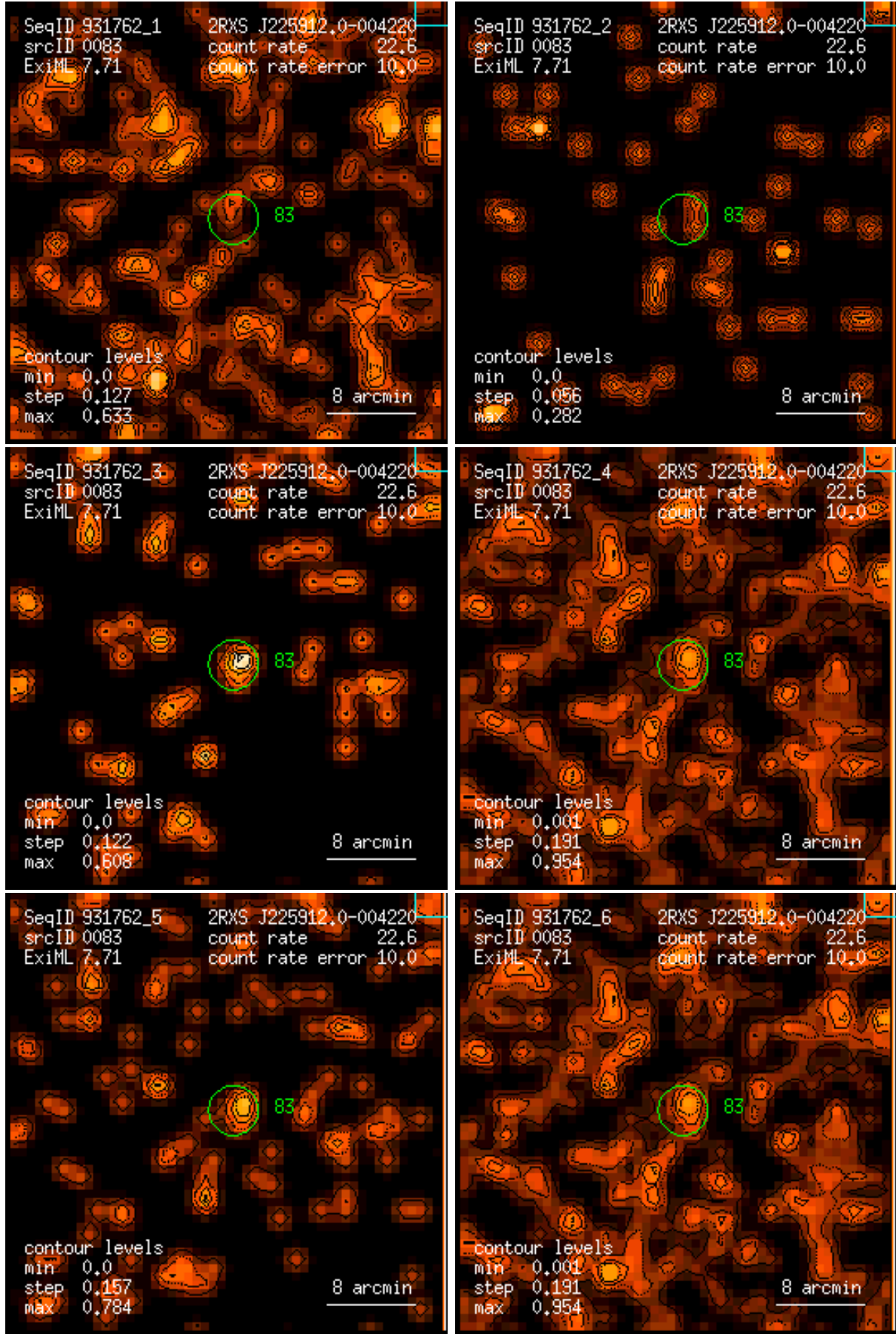
Figure 83: RASS 931762: detection 0083: band rate images, Gaussian filter: (1) PSPC channels 11 – 41, (2) 52 – 90, (3) 91 – 201, (4) 11 – 235, (5) 52 – 201, (6) 11 – 201. Broad band rates in counts/ks. Band rate contour levels in counts/ks/arcmin 2 .
