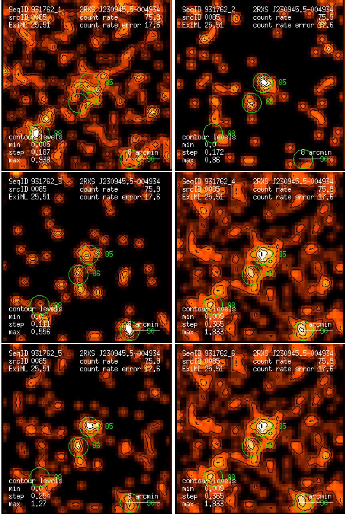
Figure 85: RASS 931762: detection 0085: band rate images, Gaussian filter: (1) PSPC channels 11 – 41, (2) 52 – 90, (3) 91 – 201, (4) 11 – 235, (5) 52 – 201, (6) 11 – 201. Broad band rates in counts/ks. Band rate contour levels in counts/ks/arcmin 2 .
