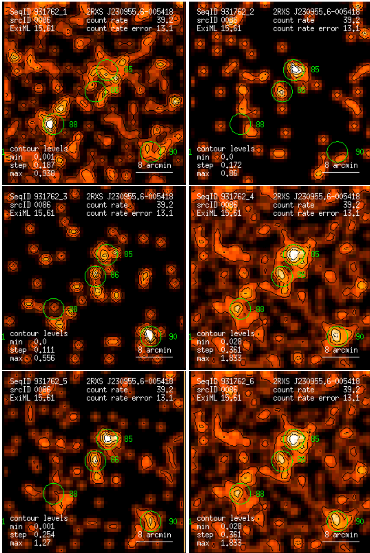
Figure 86: RASS 931762: detection 0086: band rate images, Gaussian filter: (1) PSPC channels 11 – 41, (2) 52 – 90, (3) 91 – 201, (4) 11 – 235, (5) 52 – 201, (6) 11 – 201. Broad band rates in counts/ks. Band rate contour levels in counts/ks/arcmin 2 .
