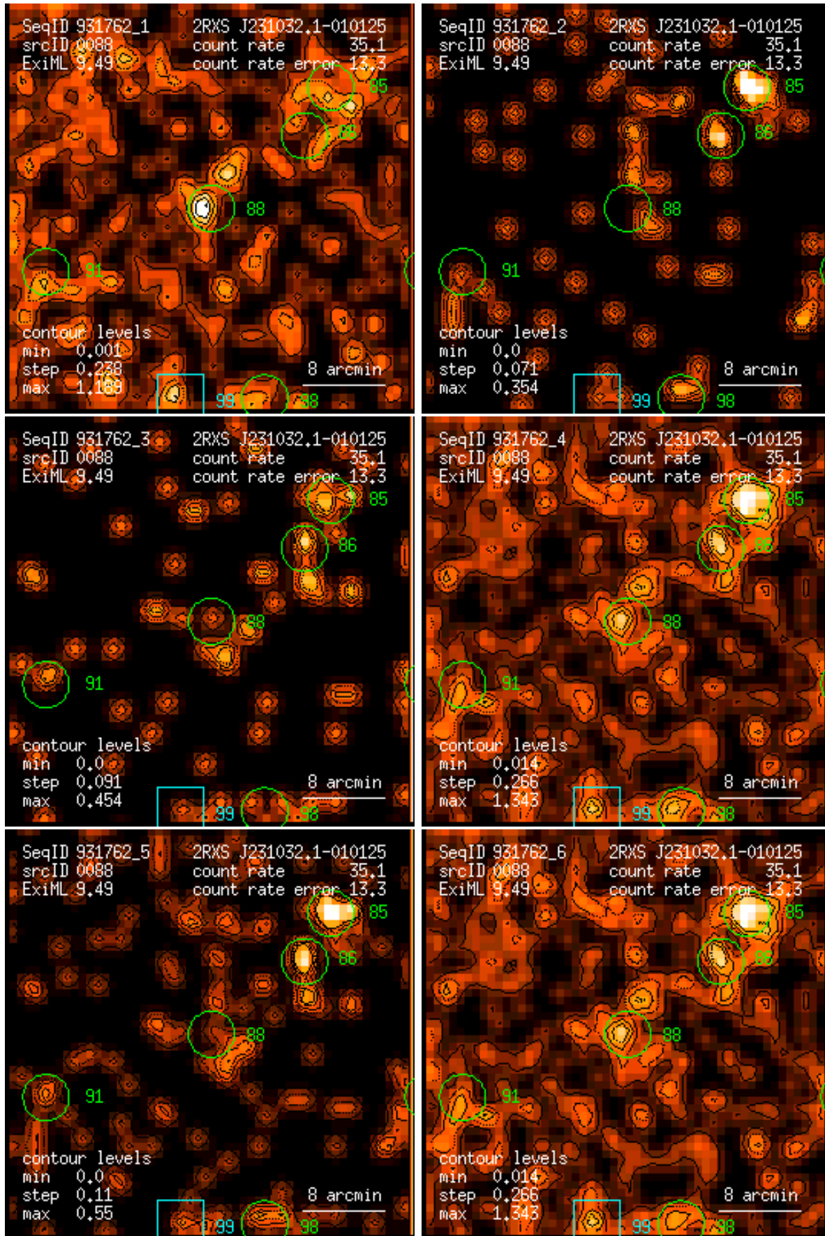
Figure 88: RASS 931762: detection 0088: band rate images, Gaussian filter: (1) PSPC channels 11 – 41, (2) 52 – 90, (3) 91 – 201, (4) 11 – 235, (5) 52 – 201, (6) 11 – 201. Broad band rates in counts/ks. Band rate contour levels in counts/ks/arcmin 2 .
