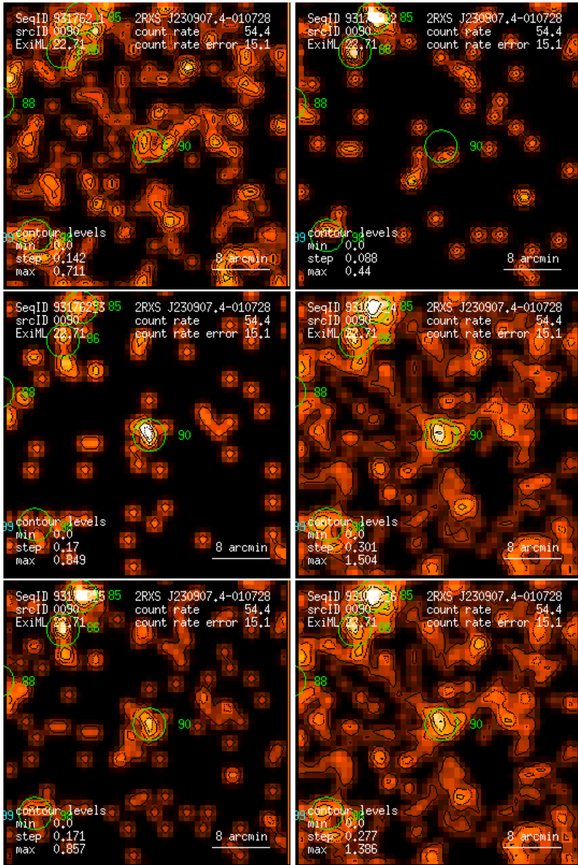
Figure 90: RASS 931762: detection 0090: band rate images, Gaussian filter: (1) PSPC channels 11 – 41, (2) 52 – 90, (3) 91 – 201, (4) 11 – 235, (5) 52 – 201, (6) 11 – 201. Broad band rates in counts/ks. Band rate contour levels in counts/ks/arcmin 2 .
