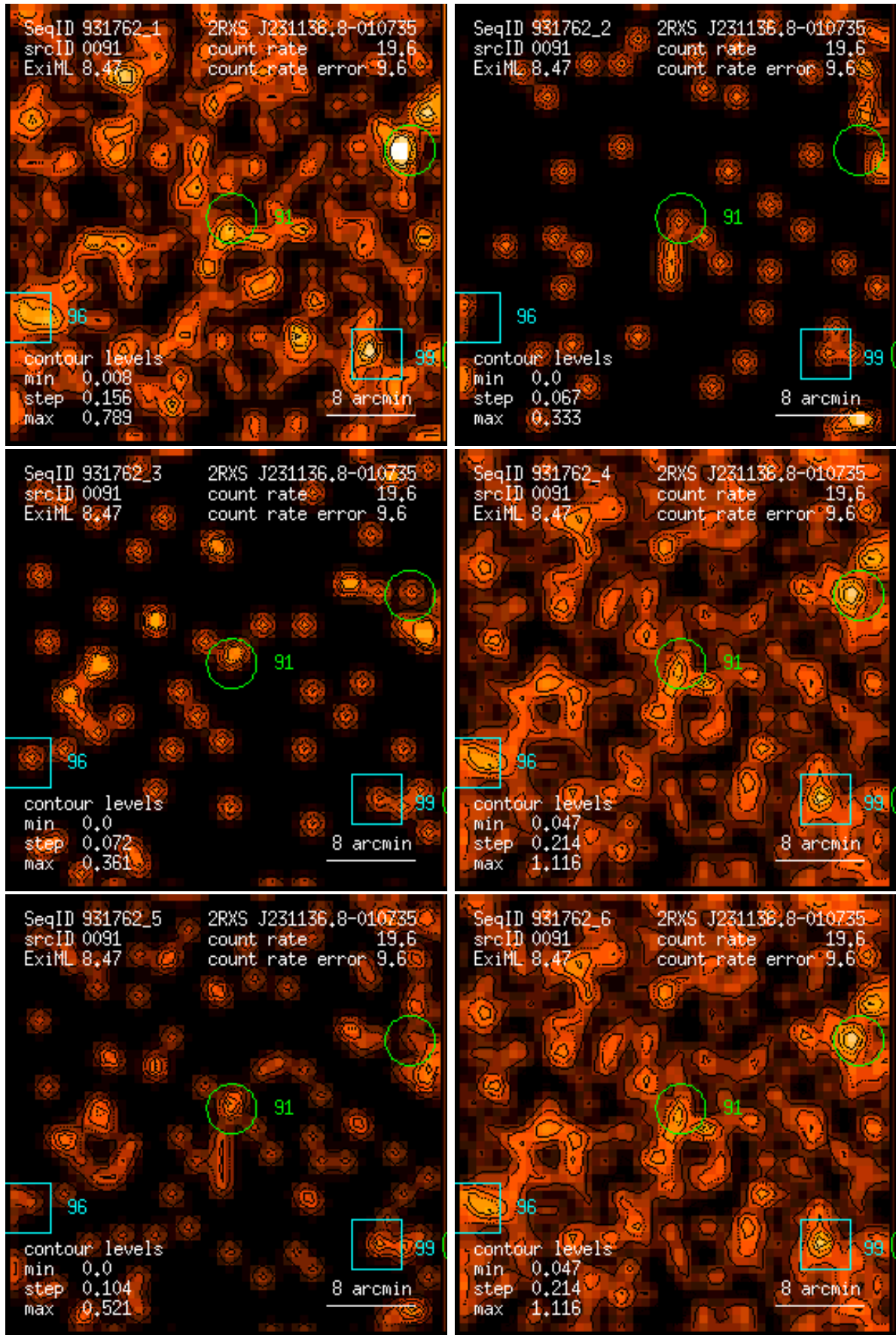
Figure 91: RASS 931762: detection 0091: band rate images, Gaussian filter: (1) PSPC channels 11 – 41, (2) 52 – 90, (3) 91 – 201, (4) 11 – 235, (5) 52 – 201, (6) 11 – 201. Broad band rates in counts/ks. Band rate contour levels in counts/ks/arcmin 2 .
