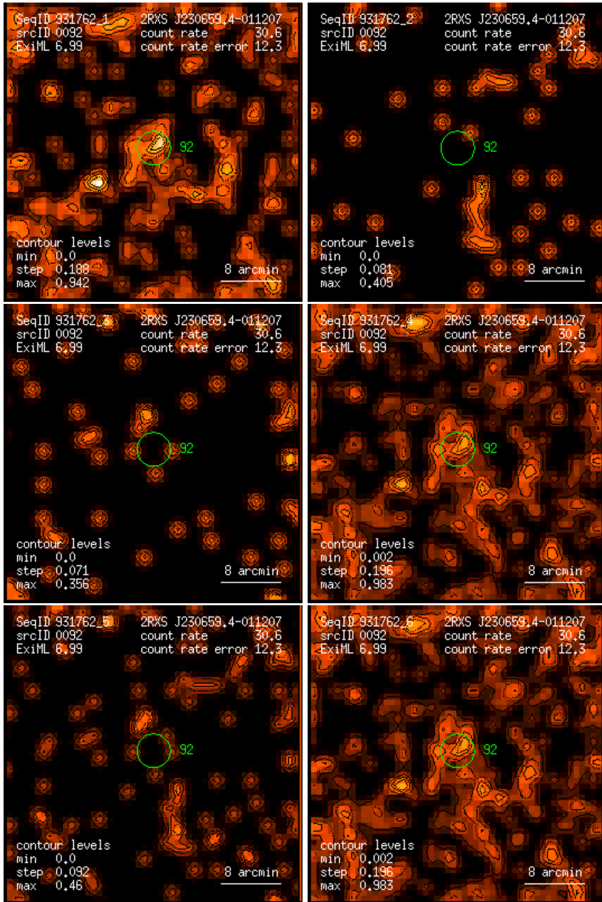
Figure 92: RASS 931762: detection 0092: band rate images, Gaussian filter: (1) PSPC channels 11 – 41, (2) 52 – 90, (3) 91 – 201, (4) 11 – 235, (5) 52 – 201, (6) 11 – 201. Broad band rates in counts/ks. Band rate contour levels in counts/ks/arcmin 2 .
