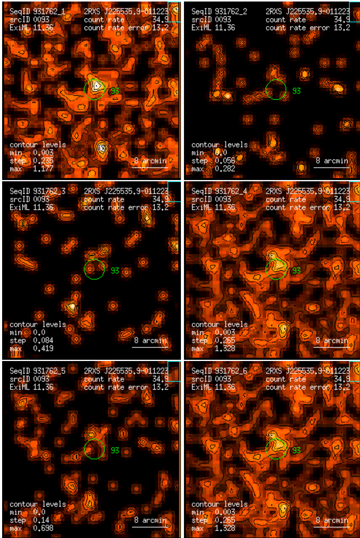
Figure 93: RASS 931762: detection 0093: band rate images, Gaussian filter: (1) PSPC channels 11 – 41, (2) 52 – 90, (3) 91 – 201, (4) 11 – 235, (5) 52 – 201, (6) 11 – 201. Broad band rates in counts/ks. Band rate contour levels in counts/ks/arcmin 2 .
