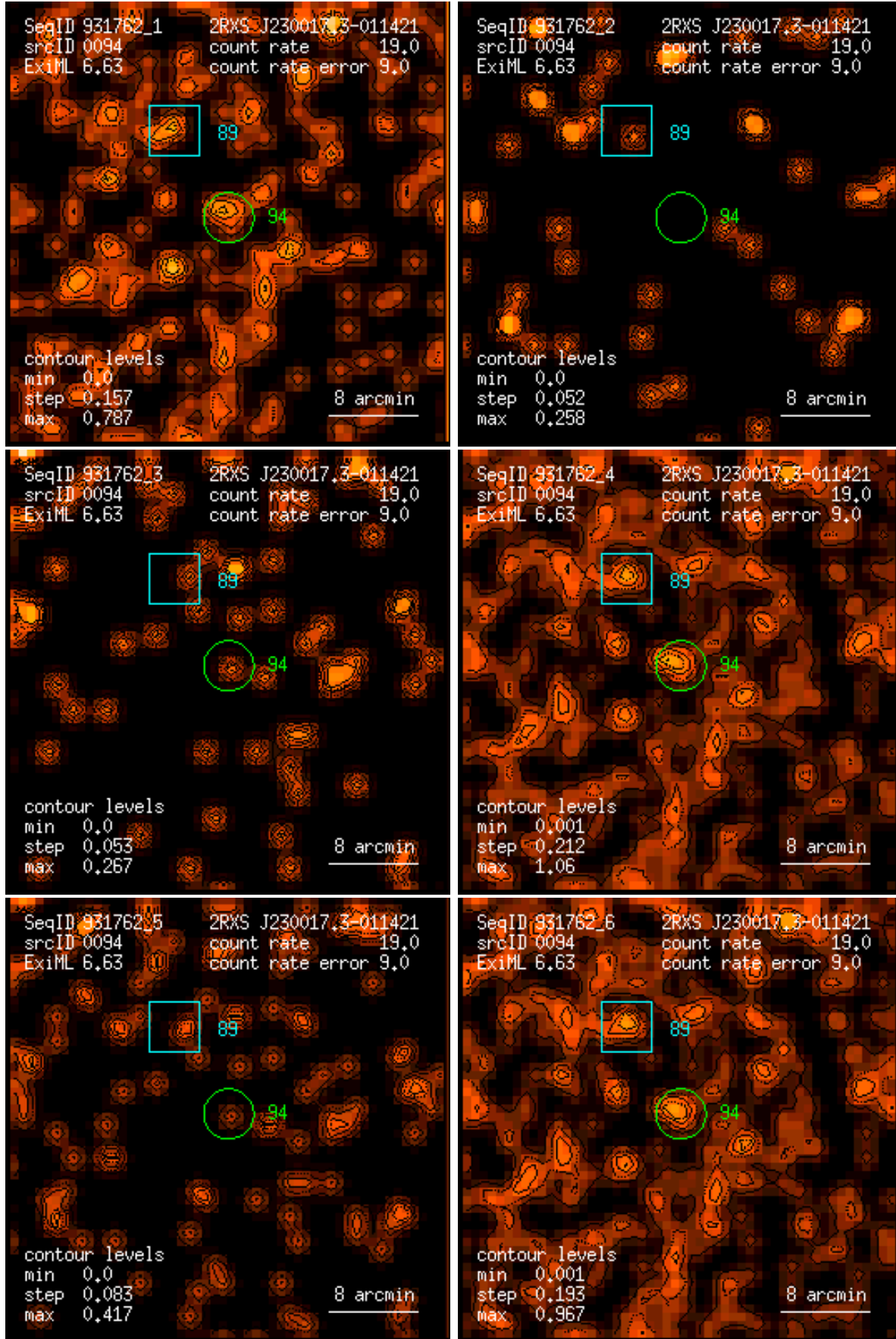
Figure 94: RASS 931762: detection 0094: band rate images, Gaussian filter: (1) PSPC channels 11 – 41, (2) 52 – 90, (3) 91 – 201, (4) 11 – 235, (5) 52 – 201, (6) 11 – 201. Broad band rates in counts/ks. Band rate contour levels in counts/ks/arcmin 2 .
