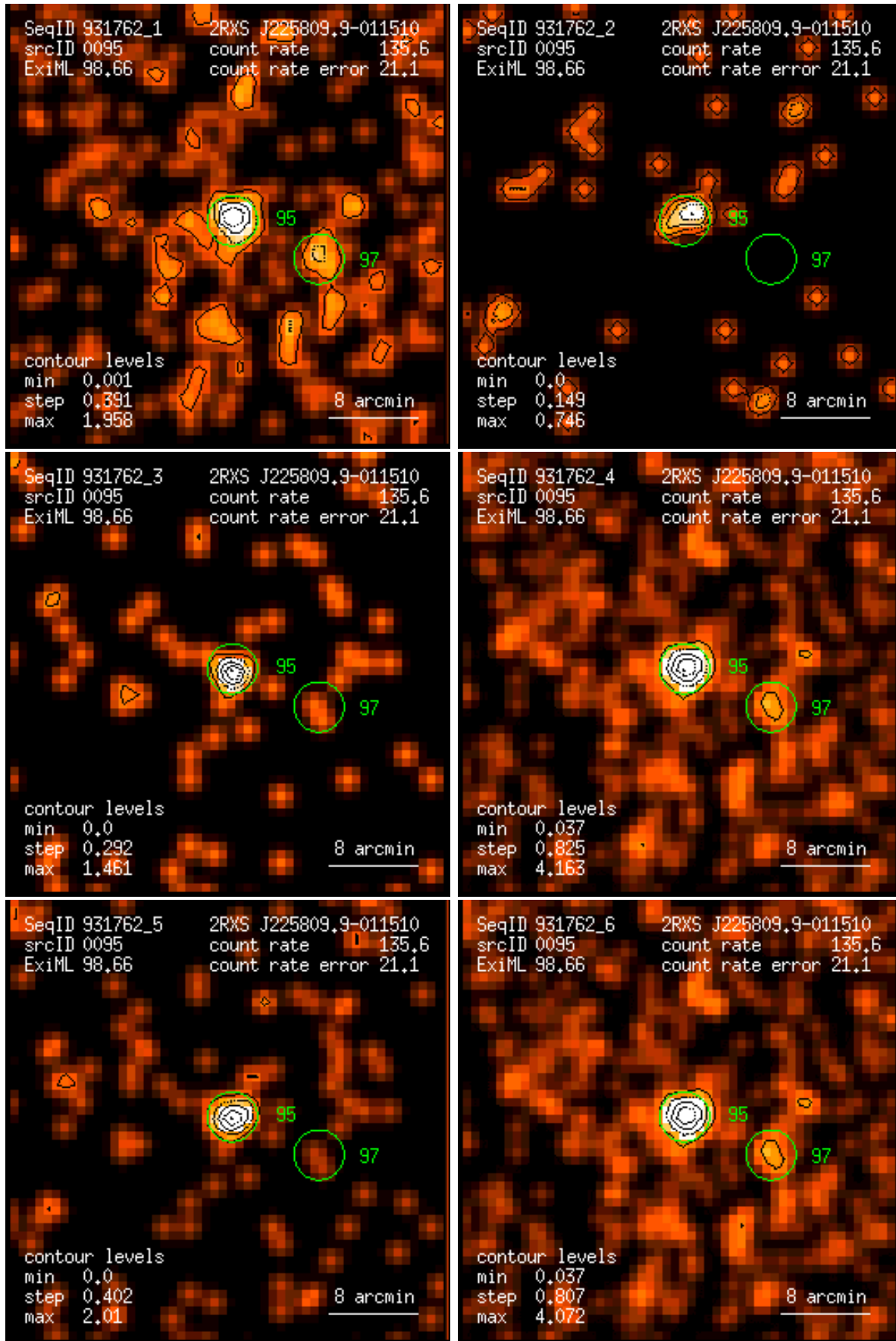
Figure 95: RASS 931762: detection 0095: band rate images, Gaussian filter: (1) PSPC channels 11 – 41, (2) 52 – 90, (3) 91 – 201, (4) 11 – 235, (5) 52 – 201, (6) 11 – 201. Broad band rates in counts/ks. Band rate contour levels in counts/ks/arcmin 2 .
