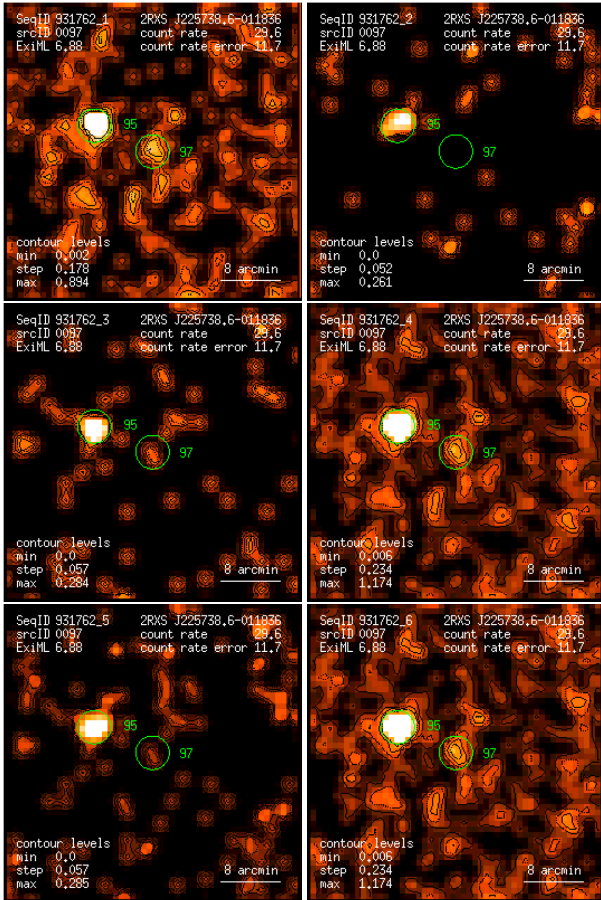
Figure 97: RASS 931762: detection 0097: band rate images, Gaussian filter: (1) PSPC channels 11 – 41, (2) 52 – 90, (3) 91 – 201, (4) 11 – 235, (5) 52 – 201, (6) 11 – 201. Broad band rates in counts/ks. Band rate contour levels in counts/ks/arcmin 2 .
