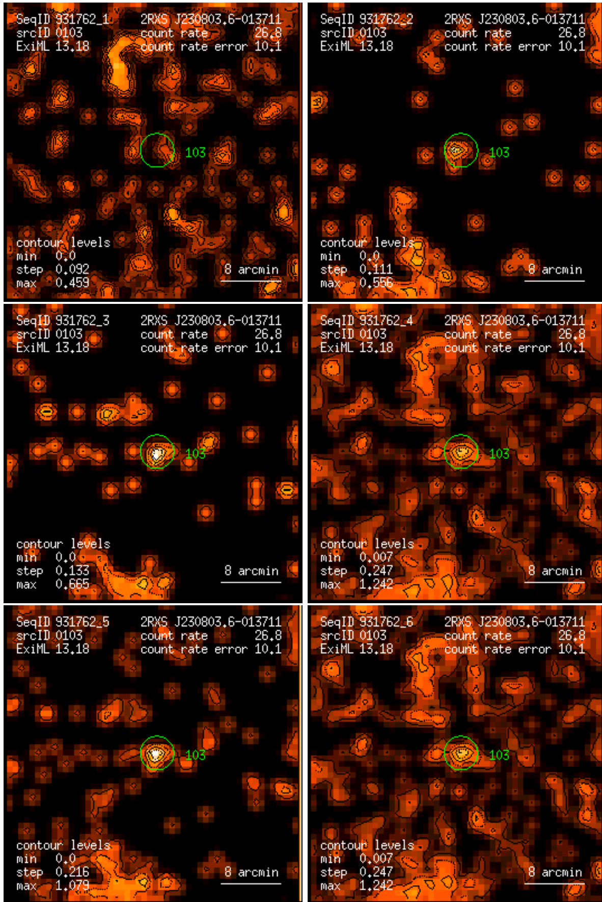
Figure 103: RASS 931762: detection 0103: band rate images, Gaussian filter: (1) PSPC channels 11 – 41, (2) 52 – 90, (3) 91 – 201, (4) 11 – 235, (5) 52 – 201, (6) 11 – 201. Broad band rates in counts/ks. Band rate contour levels in counts/ks/arcmin 2 .
