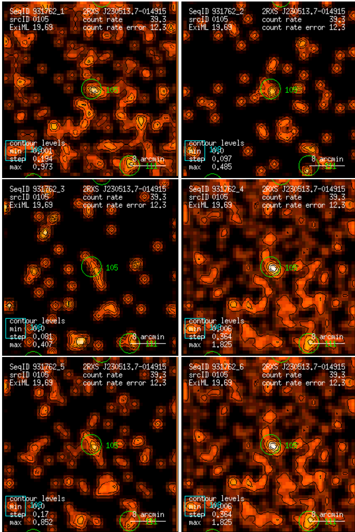
Figure 105: RASS 931762: detection 0105: band rate images, Gaussian filter: (1) PSPC channels 11 – 41, (2) 52 – 90, (3) 91 – 201, (4) 11 – 235, (5) 52 – 201, (6) 11 – 201. Broad band rates in counts/ks. Band rate contour levels in counts/ks/arcmin 2 .
