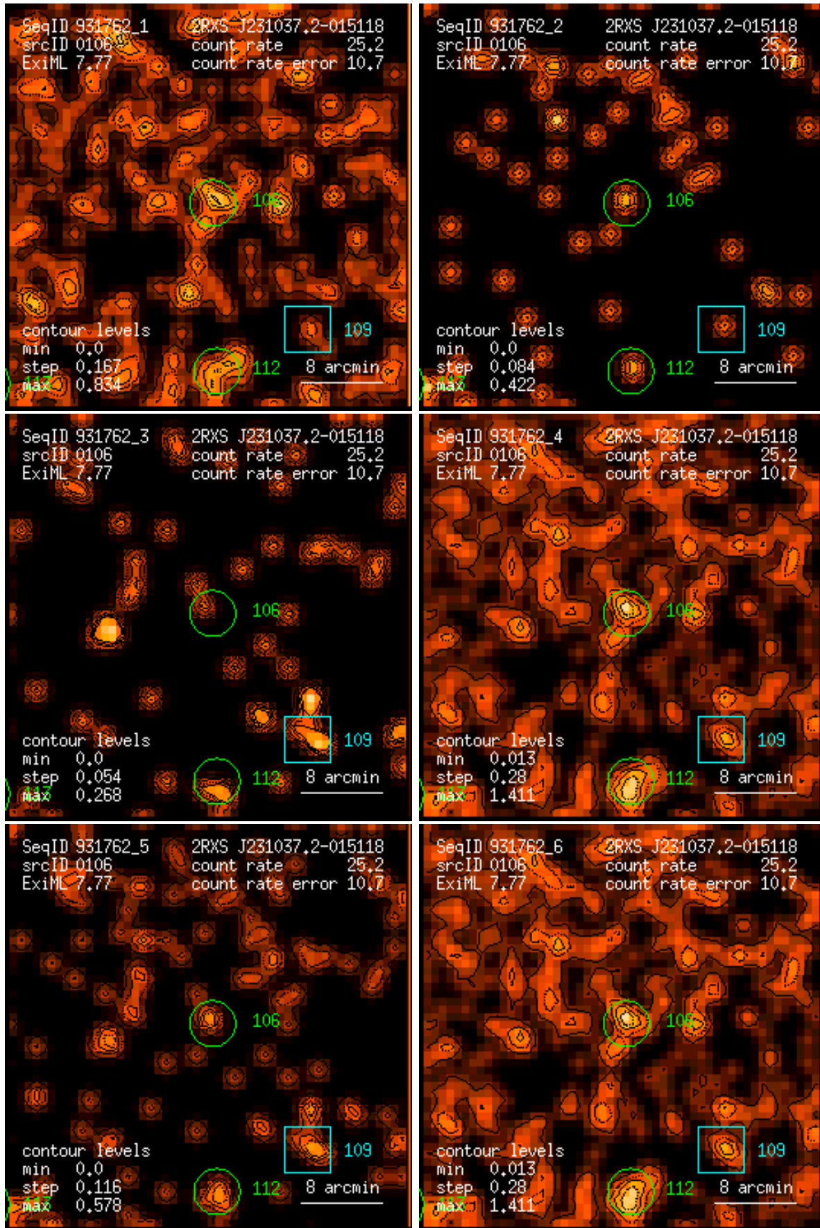
Figure 106: RASS 931762: detection 0106: band rate images, Gaussian filter: (1) PSPC channels 11 – 41, (2) 52 – 90, (3) 91 – 201, (4) 11 – 235, (5) 52 – 201, (6) 11 – 201. Broad band rates in counts/ks. Band rate contour levels in counts/ks/arcmin 2 .
