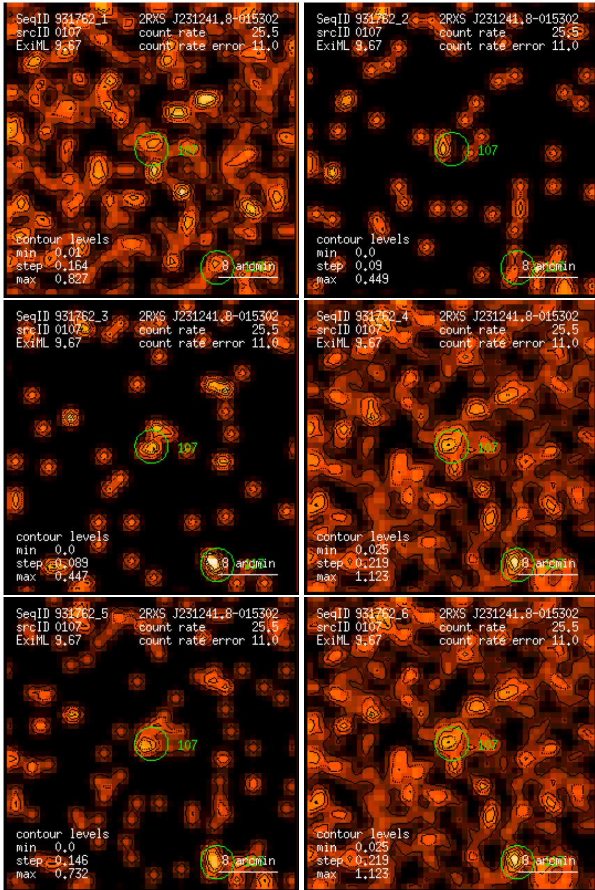
Figure 107: RASS 931762: detection 0107: band rate images, Gaussian filter: (1) PSPC channels 11 – 41, (2) 52 – 90, (3) 91 – 201, (4) 11 – 235, (5) 52 – 201, (6) 11 – 201. Broad band rates in counts/ks. Band rate contour levels in counts/ks/arcmin 2 .
