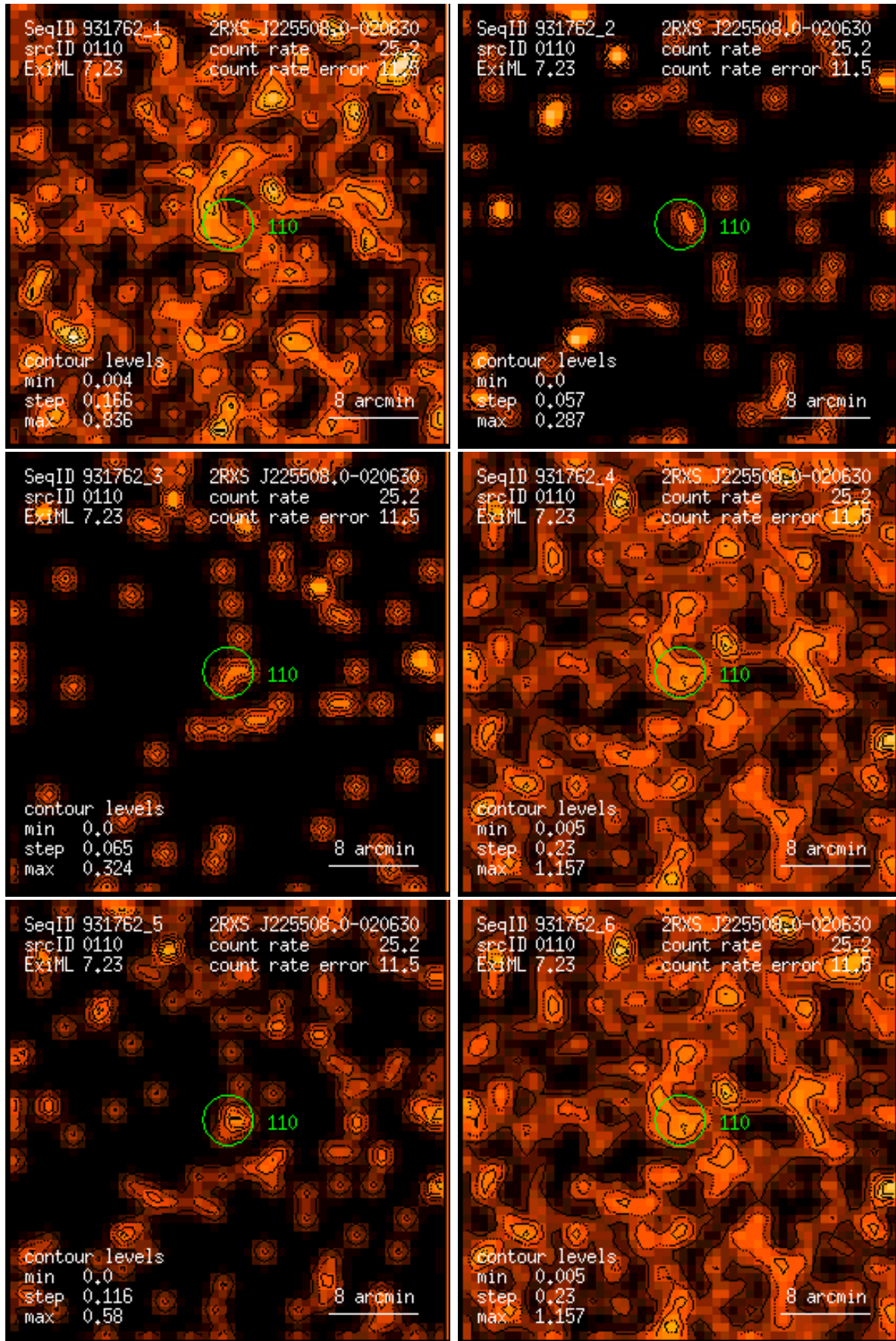
Figure 110: RASS 931762: detection 0110: band rate images, Gaussian filter: (1) PSPC channels 11 – 41, (2) 52 – 90, (3) 91 – 201, (4) 11 – 235, (5) 52 – 201, (6) 11 – 201. Broad band rates in counts/ks. Band rate contour levels in counts/ks/arcmin 2 .
