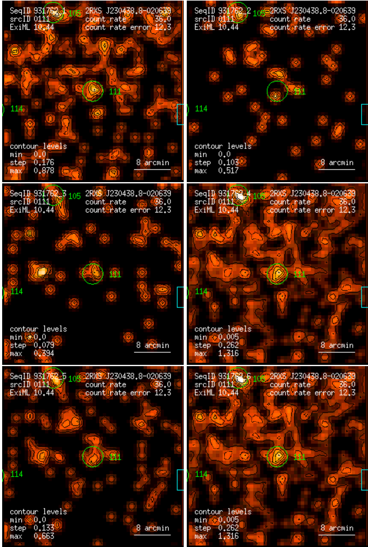
Figure 111: RASS 931762: detection 0111: band rate images, Gaussian filter: (1) PSPC channels 11 – 41, (2) 52 – 90, (3) 91 – 201, (4) 11 – 235, (5) 52 – 201, (6) 11 – 201. Broad band rates in counts/ks. Band rate contour levels in counts/ks/arcmin 2 .
