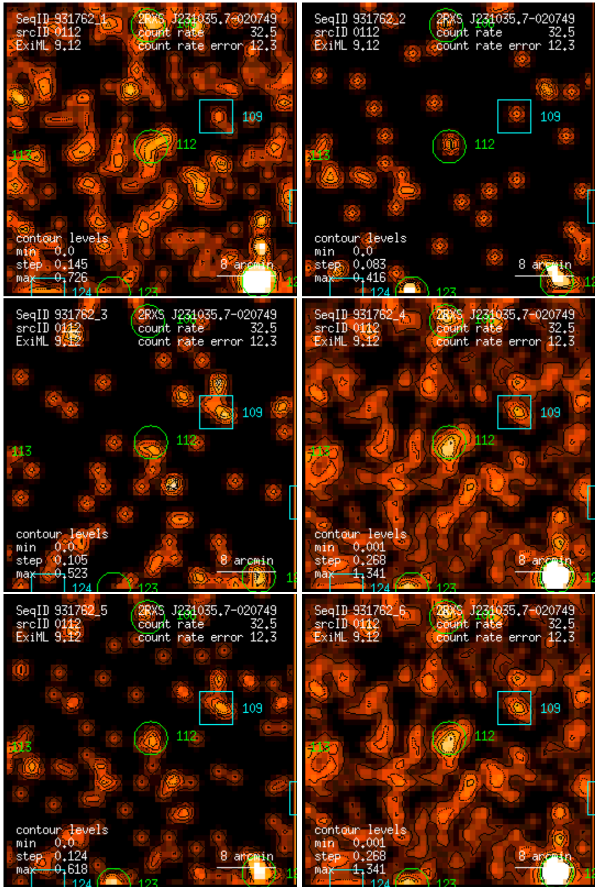
Figure 112: RASS 931762: detection 0112: band rate images, Gaussian filter: (1) PSPC channels 11 – 41, (2) 52 – 90, (3) 91 – 201, (4) 11 – 235, (5) 52 – 201, (6) 11 – 201. Broad band rates in counts/ks. Band rate contour levels in counts/ks/arcmin 2 .
